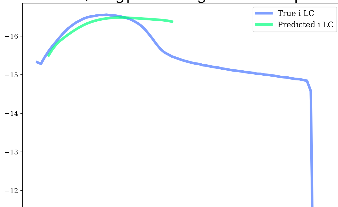
i-band, Avg|Max Mag Diff: 0.24 | 0.9
