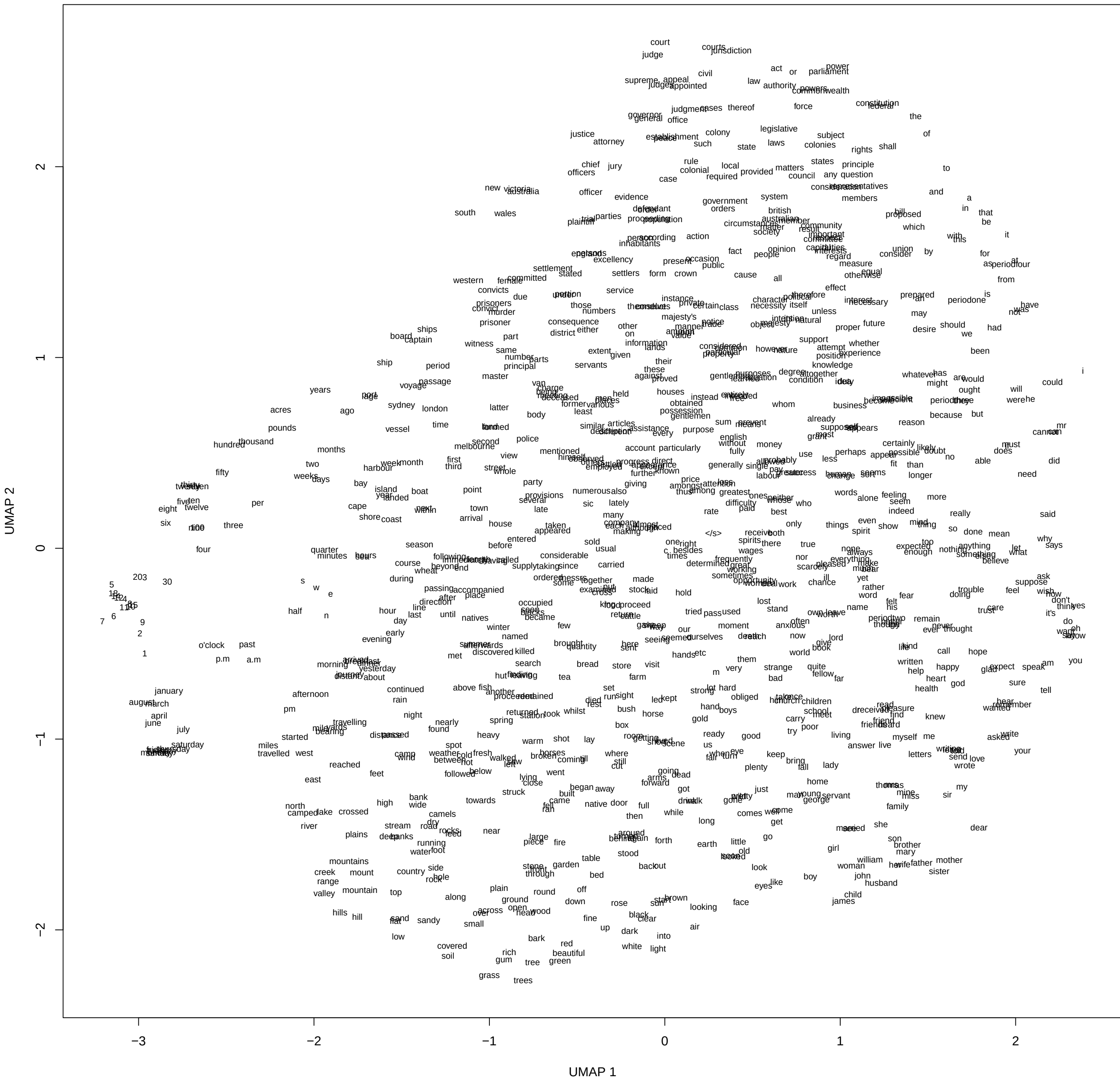
UMAP projection
