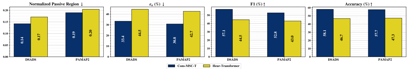
Fig. 12: Comparing the Cons-MSC-T approach (blue) to the approach from [42] (yellow) on the DSADS and PAMAP2 benchmarks. We consider the passive region and active error rate to evaluate the policy and classifier respectively. We also show the overall F1-score and accuracy.
