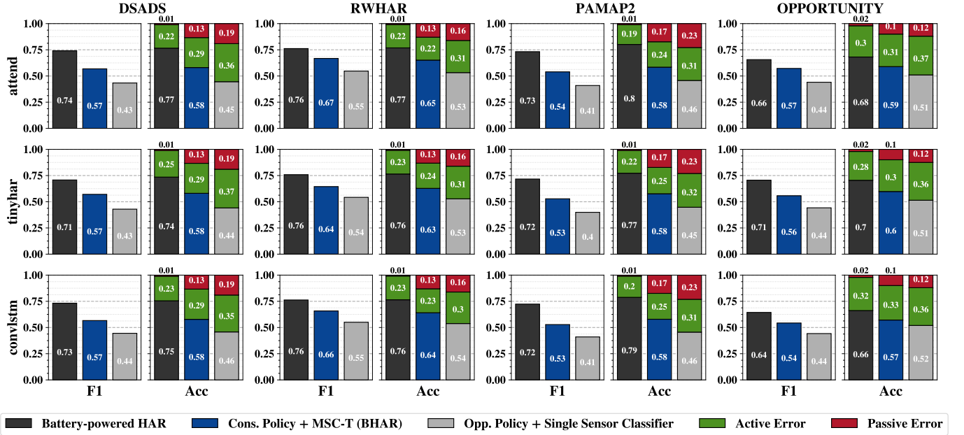
Fig. 6: F1-score and accuracy breakdown. Each row (e.g. attend, etc.) is an architecture while each pair of columns shows the F1-score ( F1 ) and accuracy ( Acc ) for each dataset (e.g. DSADS, etc.). The black and gray bars show the upper and lower bound baselines, respectively, while the blue bars show Cons-MSC-T. The error (green + red bars) and accuracy add to 1 as shown by the stacked bars reaching 1 in the Acc columns. The reduction in active (green) and passive (red) errors reflects improvements in the classifier and the policy, respectively. Opp. and Cons. stand for Opportunistic and Conservative, respectively.
