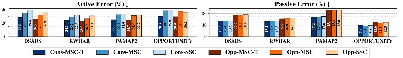
Fig. 9: Active (left) and Passive (Right) Errors for all policy-classifier combinations. For each policy (color) group, active error decreases as we progress from SSC to MSC to MSC-T. Conversely, conservative approaches (blue) have a smaller passive error than the opportunistic approaches (orange)
