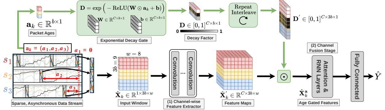
Fig. 2: Multisensor Classifier with Time Context (MSC-T). We show the data flow of asynchronous data for HAR classifiers. The bottom path (black arrows) shows how the input \hat{\mathbf{X}}_k flows in existing HAR architectures with red, yellow, and blue colors corresponding to channels from sensors s_1 , s_2 , and s_3 , respectively. The top path (green arrows/boxes), shows how we integrate temporal context \mathbf{a}_k to modulate the feature maps. Darker black boxes in the decay factor \mathbf{D} show how stale data will be scaled to zero while lighter white boxes show how fresh data will be passed through.
