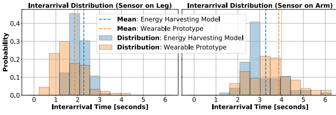
Fig. 5: Interarrival time distribution of energy harvesting model (blue) and prototype (orange) while walking. The similarity between the distributions reflects that the harvesting model provides a practical estimate of harvested energy.
