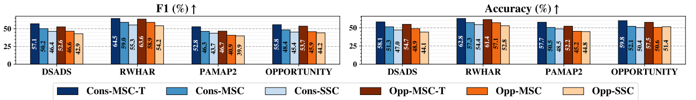
Fig. 10: F1-score (left) and Accuracy (right) for all policy-classifier combinations. Across all datasets, we see that the Cons-MSC-T approach achieves the highest F1-score and accuracy.
