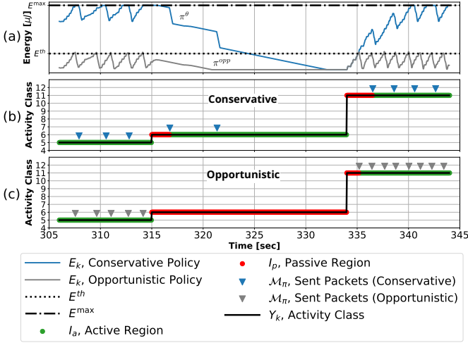
Fig. 3: (a) Energy level E_k for two policies. The dotted line is the threshold E^{Th} needed to send a packet. The dashed line is the max energy E^{max} . The opportunistic policy (gray), \pi^{opp} , transmits when E_k > E^{Th} . The conservative policy (blue), \pi^\theta , saves an energy surplus. (b, c) The active I_a (green) and passive I_p (red) regions of \pi^\theta and \pi^{opp} , respectively. The packet transmission times, \mathcal{M} , are shown as triangles. During a low motion activity (315 – 334 sec), we have E_k^H < E^L so E_k decays. Thus, \pi^{opp} cannot send packets while \pi^\theta uses its surplus, resulting in a large and small I_p , respectively.
