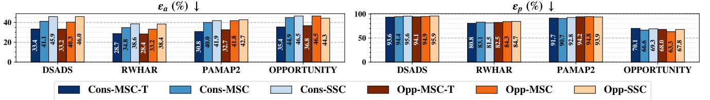
Fig. 8: Active (left) and Passive (right) Error Rates for all policy-classifier combinations. For each policy group, the MSC-T approaches achieve a lower active error rate ( \epsilon_a ) than the MSC approaches, which achieve a lower \epsilon_a than the SSC approaches.
