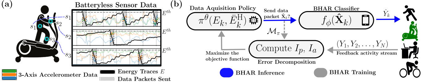
Fig. 1: (a) Batteryless HAR setting. A user wears b = 3 batteryless sensors ( s_1, s_2, s_3 ) which harvest energy from motion and output 3D acceleration (blue, orange, green signals). The black lines show the energy level of each sensor, which accumulates and then depletes when reaching the threshold E^{Th} for data acquisition (dashed line). The gray boxes show transmitted packets. (b) Batteryless HAR optimization problem. Each sensor has a policy \pi^\theta to determine when to send packets \hat{X}_k to the classifier f_\phi . The classifier runs on a smartphone to aggregate data from all sensors and outputs predictions \hat{Y}_k (e.g., run, walk). Using labels (Y_1, \dots, Y_N) and sent packets \mathcal{M}_\pi , we split the error into passive ( I_p ) and active ( I_a ) components tied to the policy and classifier. Unlike prior works, we optimize data acquisition and classification. See section III for the fully defined notation.
