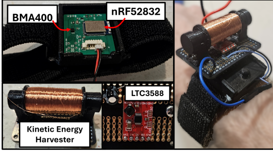
Fig. 4: Hardware prototype. (Top Left) The PCB with a BMA400 accelerometer and nRF52832 BLE MCU in a wearable case. (Bottom Left) The KEH: a wound coil with a magnetic core moving inside. (Bottom Middle) The LTC3588 PMIC: rectifies the AC voltage from the KEH to charge a 10uF capacitor, and regulates the voltage to 1.8V to power the PCB. (Right) The integrated prototype worn on the wrist.
