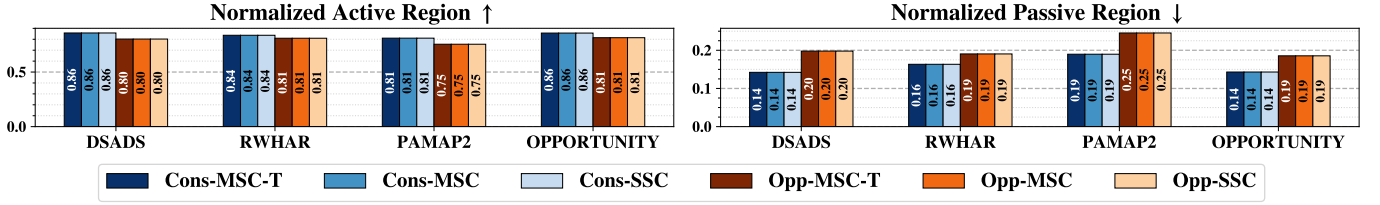
Fig. 7: Normalized Active (left) and Passive (right) Regions for all policy-classifier combinations. The normalized active region is larger (normalized passive region is lower ) for the conservative (blue) relative to the opportunistic approaches (orange).
