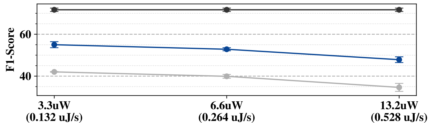
(c) Idle + Policy Energy E^L
