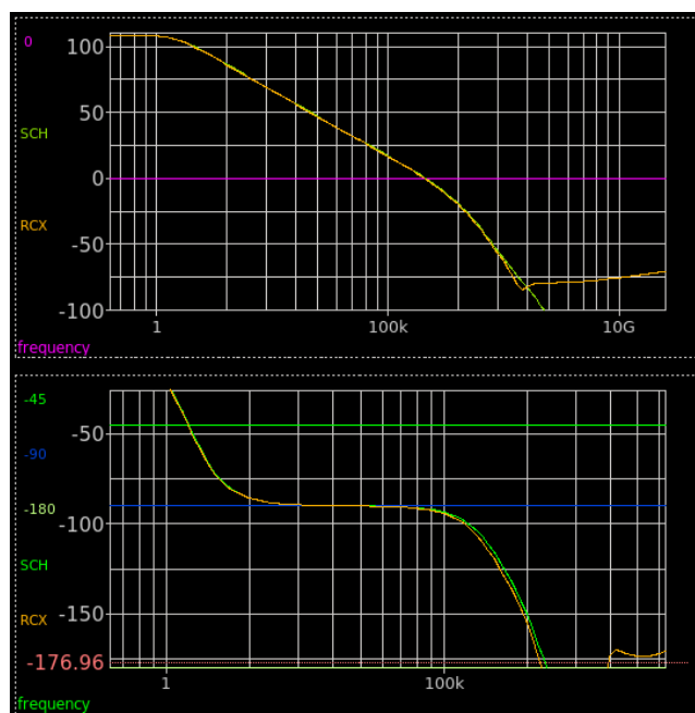
Figure 11 Pre (SCH) and post (RCX) layout stb plots
