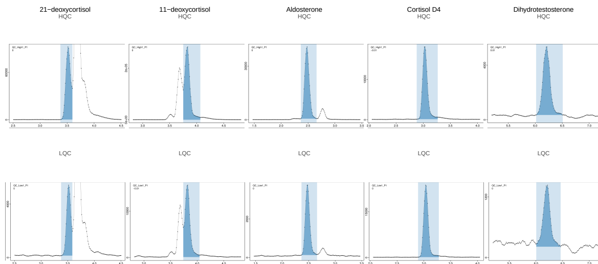
Figure 1: Example INTEGRATOR chromatograms. MRMhub-INTEGRATOR chromatograms for 21-deoxycortisol, 11-deoxycortisol, Aldosterone, Cortisol D4 (internal standard) and Dihydrotestosterone at high (HQC) and low (LQC) QC levels; the shaded region is the integrated peak.
