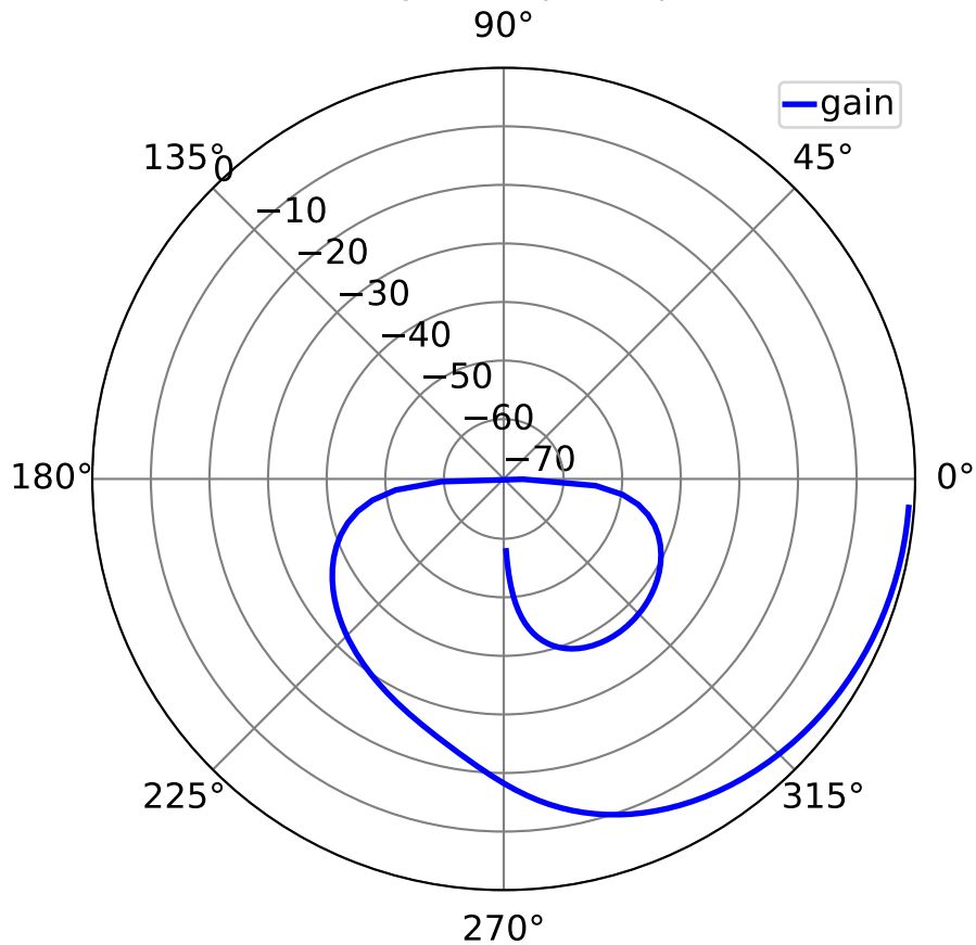
dB magnitude-phase plot
