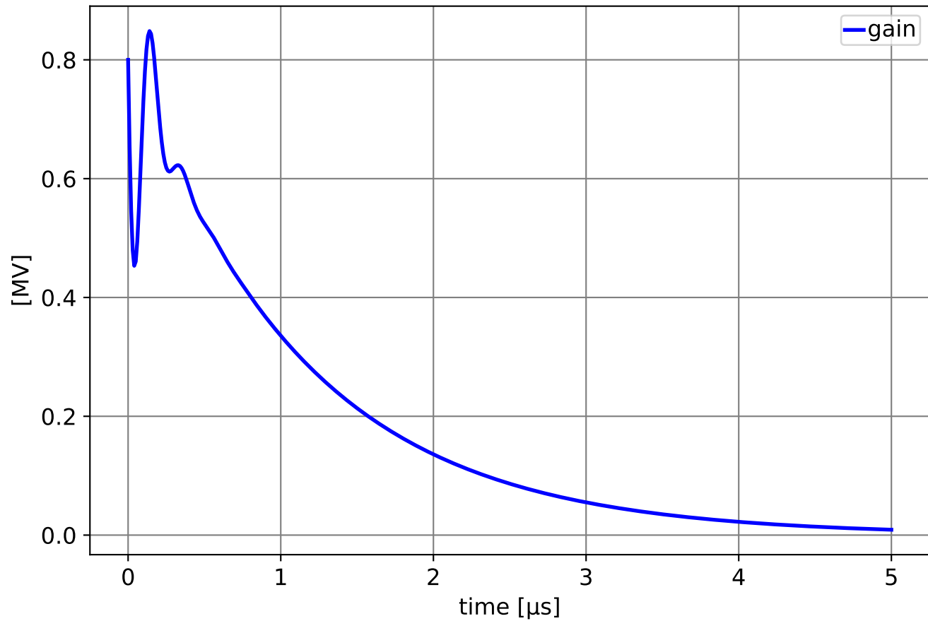
Unit-impulse response
