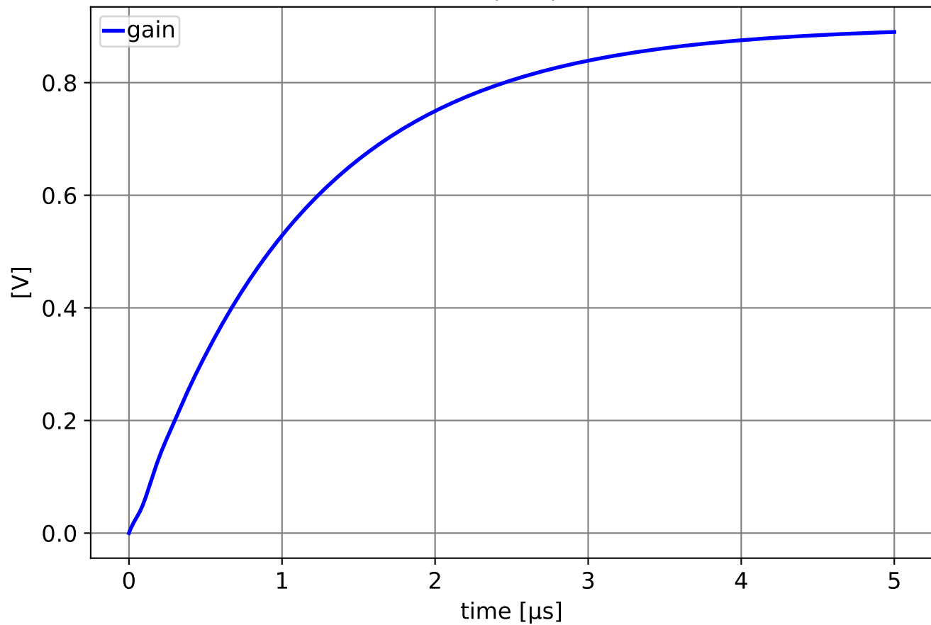
Unit-step response
