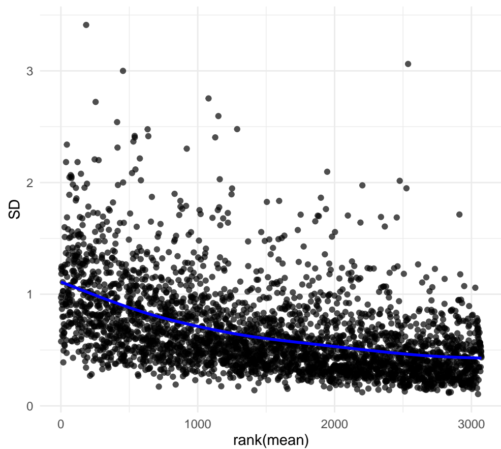
meanSdPlot – After VSN
