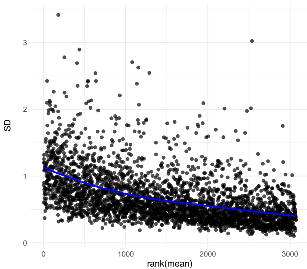
meanSdPlot – Before VSN
