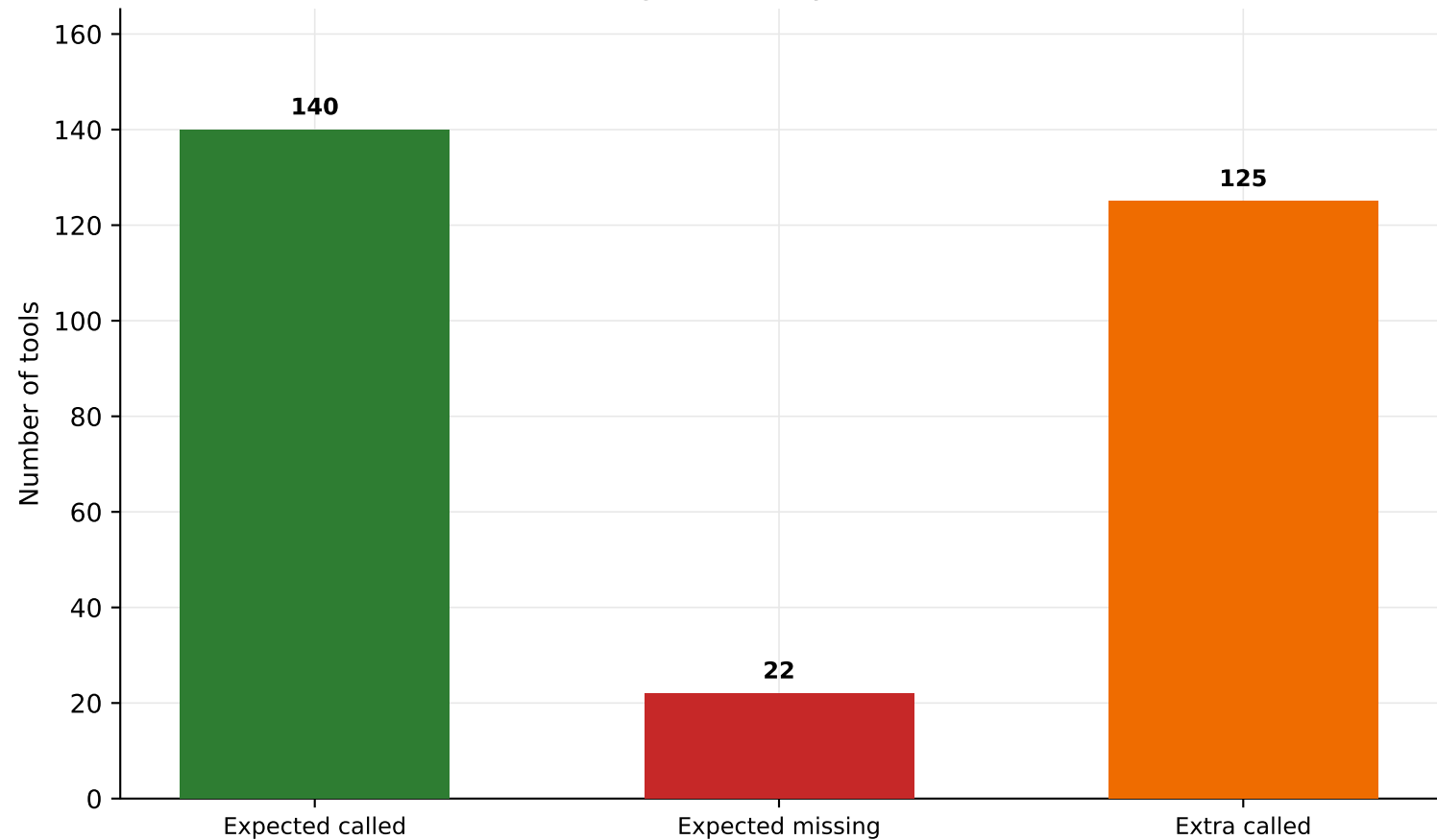
Tool usage summary - MiniMax-M3
