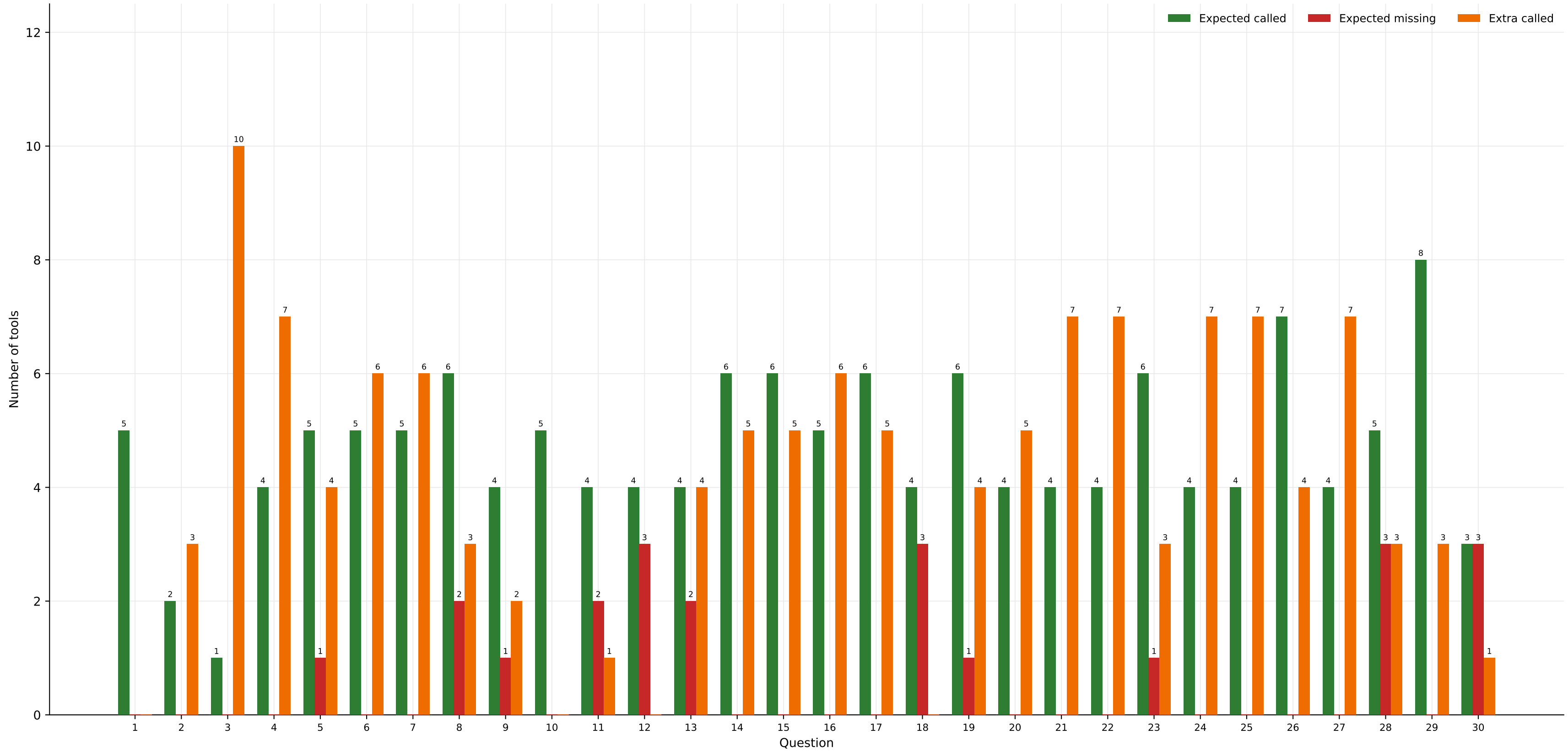
Tool usage by question - MiniMax-M3
