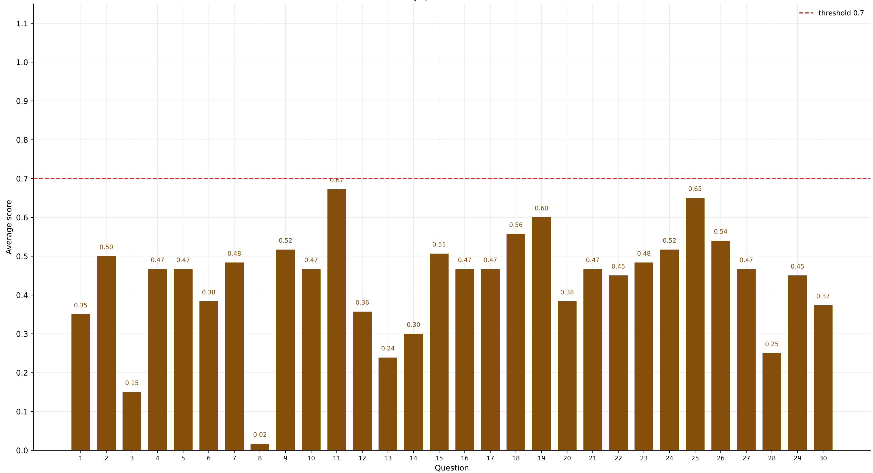
Score by question - MiniMax-M3
