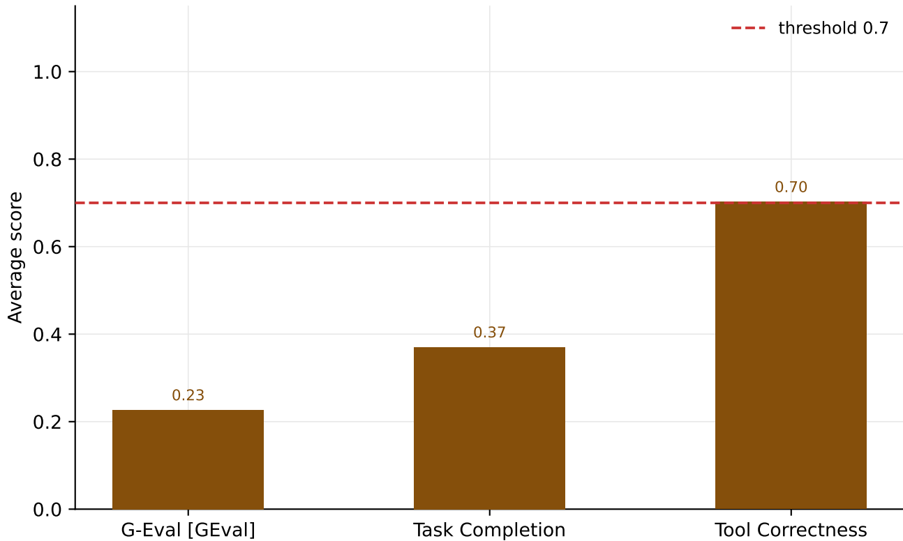
Average score by metric - MiniMax-M3
