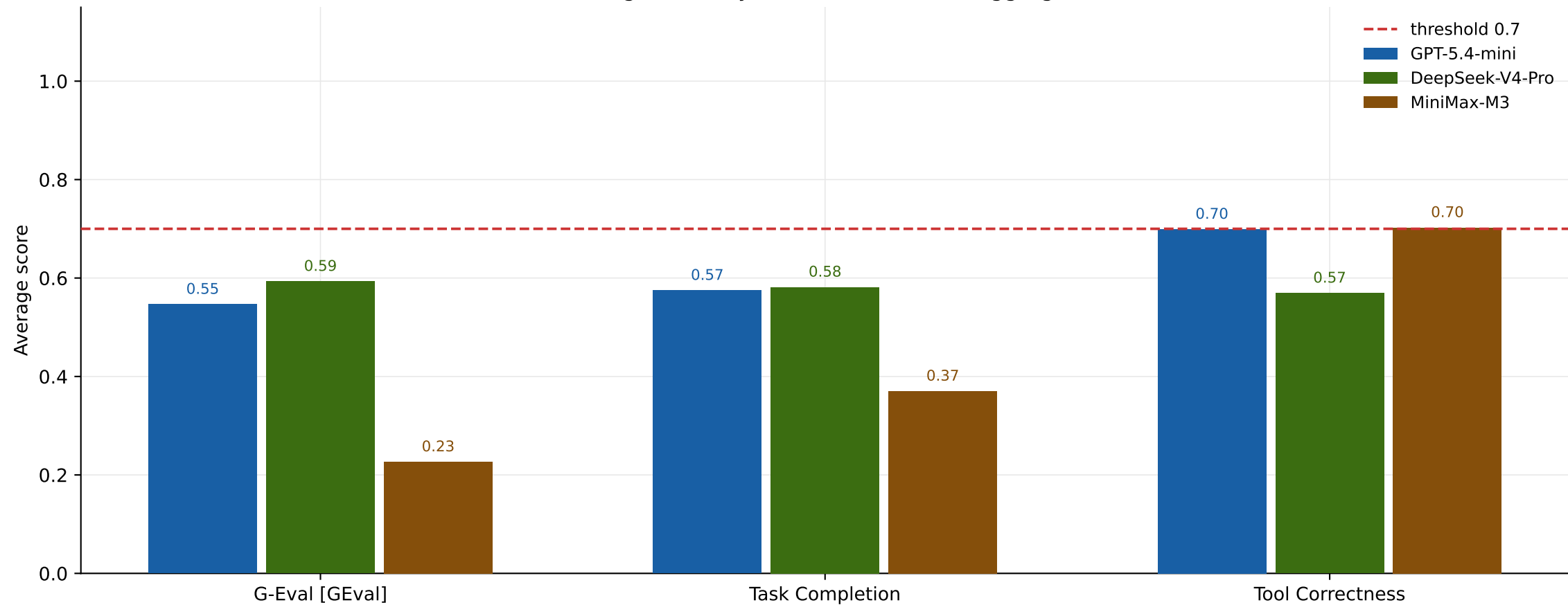
Average score by metric and model - aggregate
