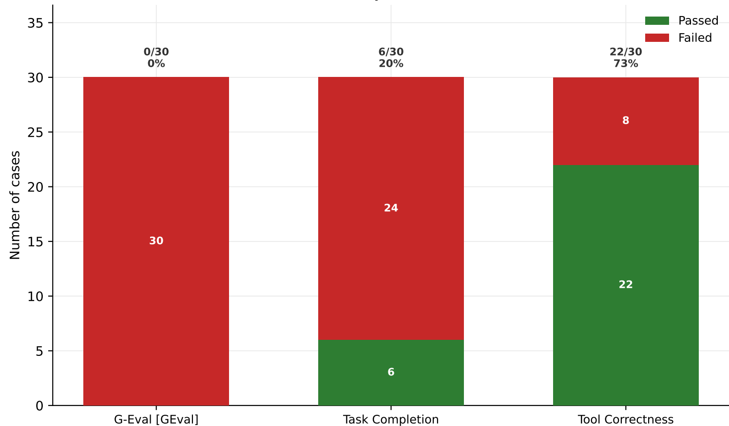
Passed vs failed by metric - MiniMax-M3
