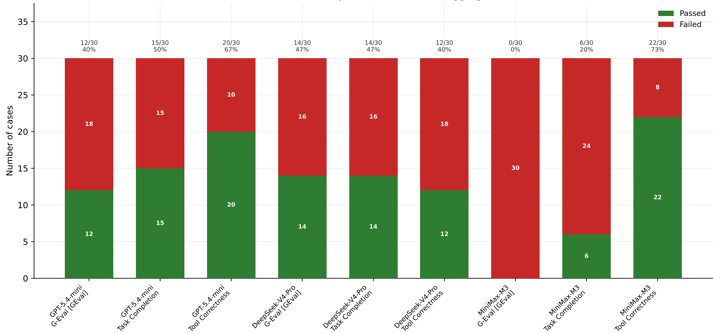
Passed vs failed by metric and model - aggregate
