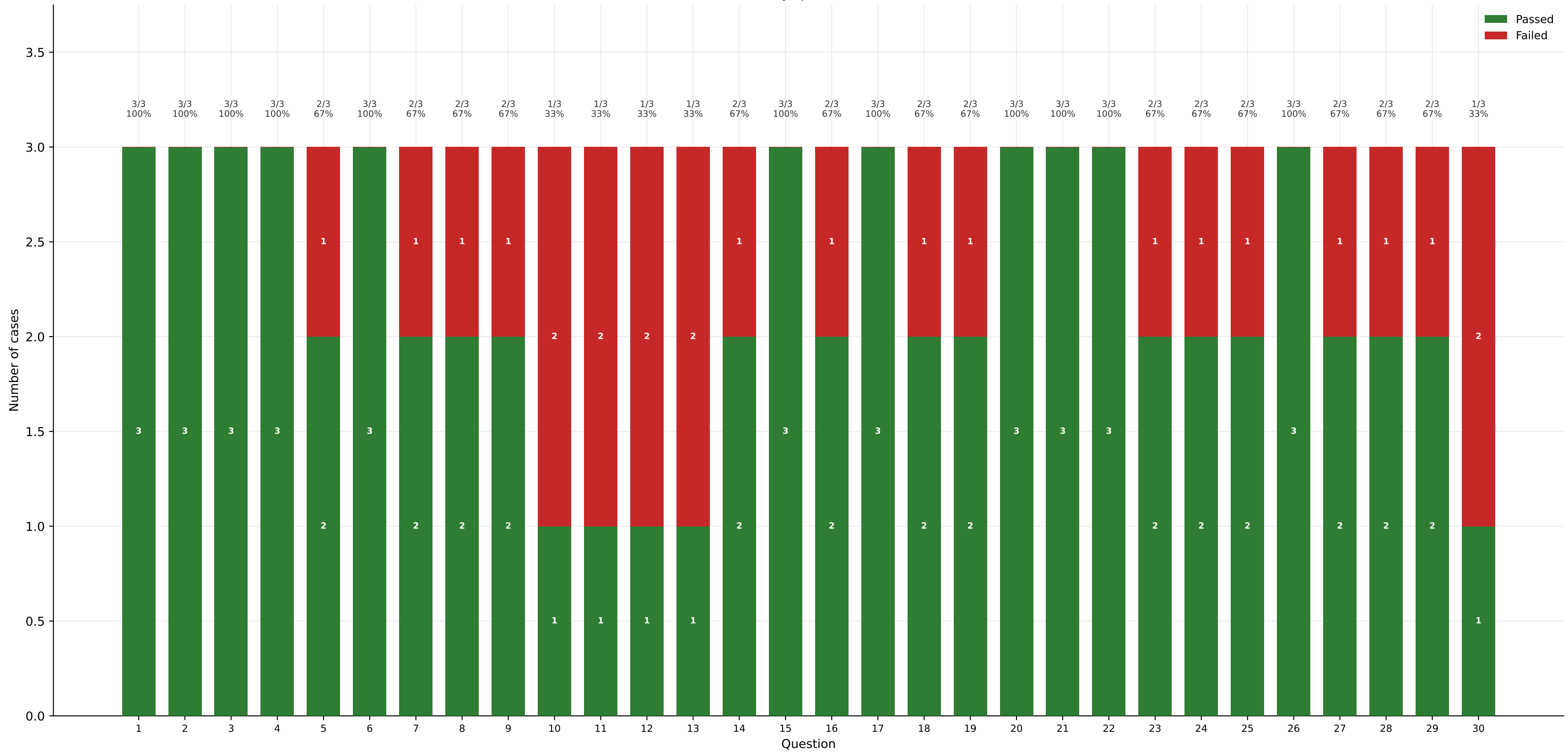
Passed vs failed by question - GPT-5.4-mini
