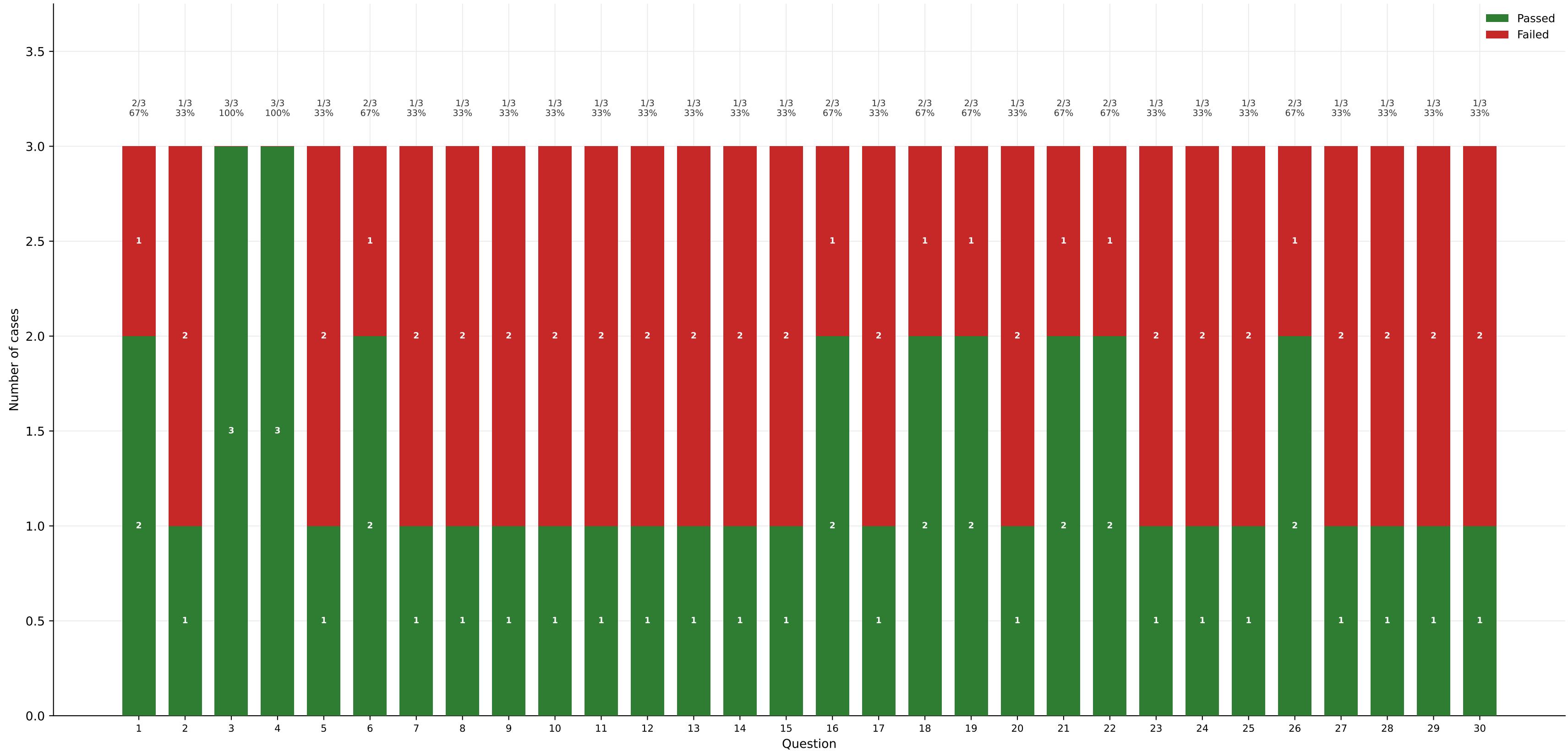
Passed vs failed by question - DeepSeek-V3.2
