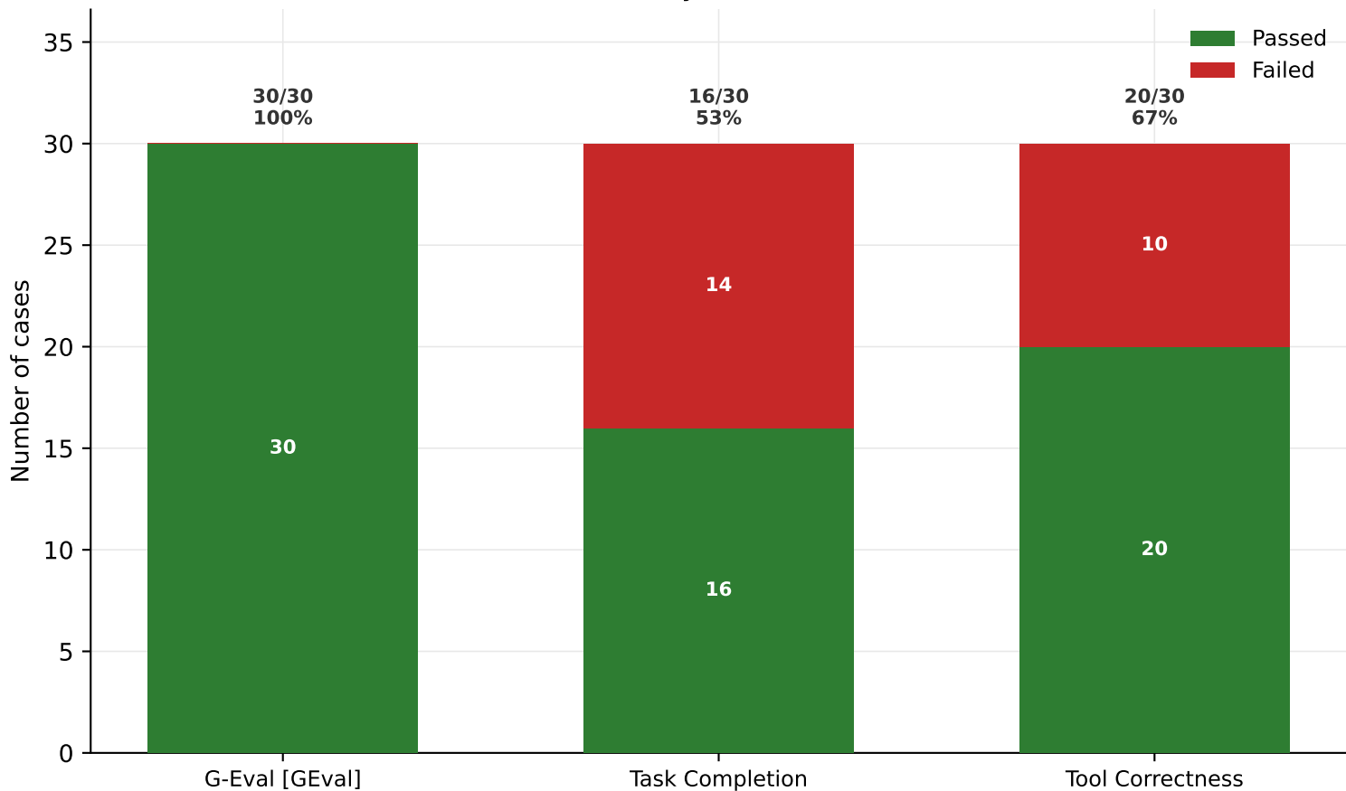
Passed vs failed by metric - GPT-5.4-mini
