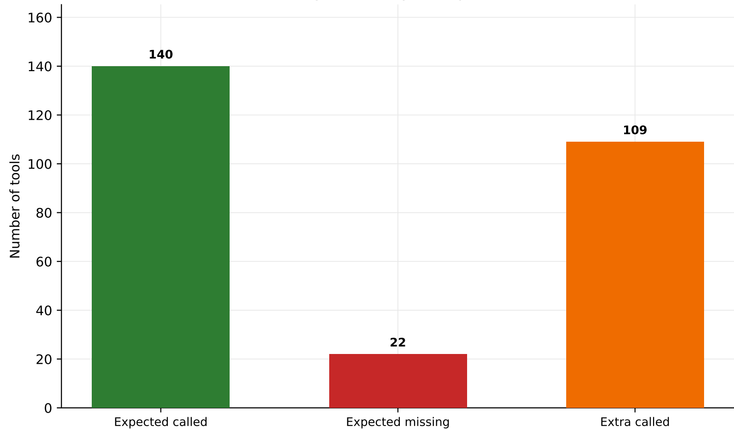
Tool usage summary - DeepSeek-V3.2
