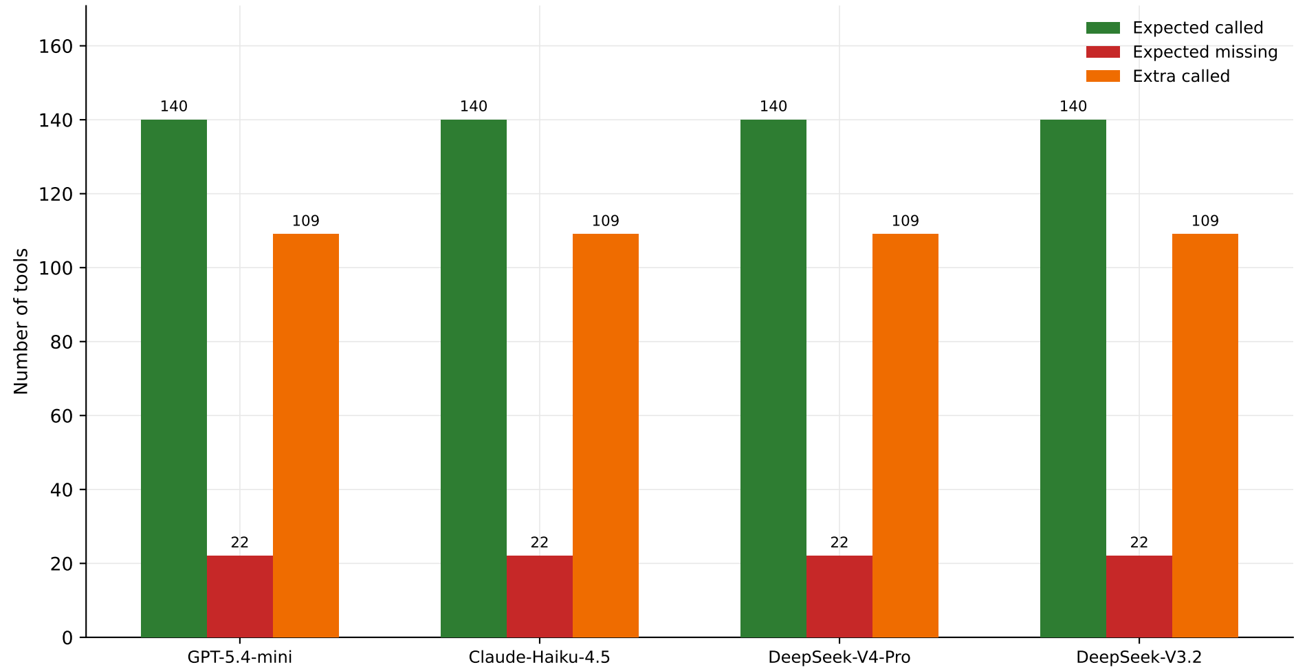
Tool usage summary by model
