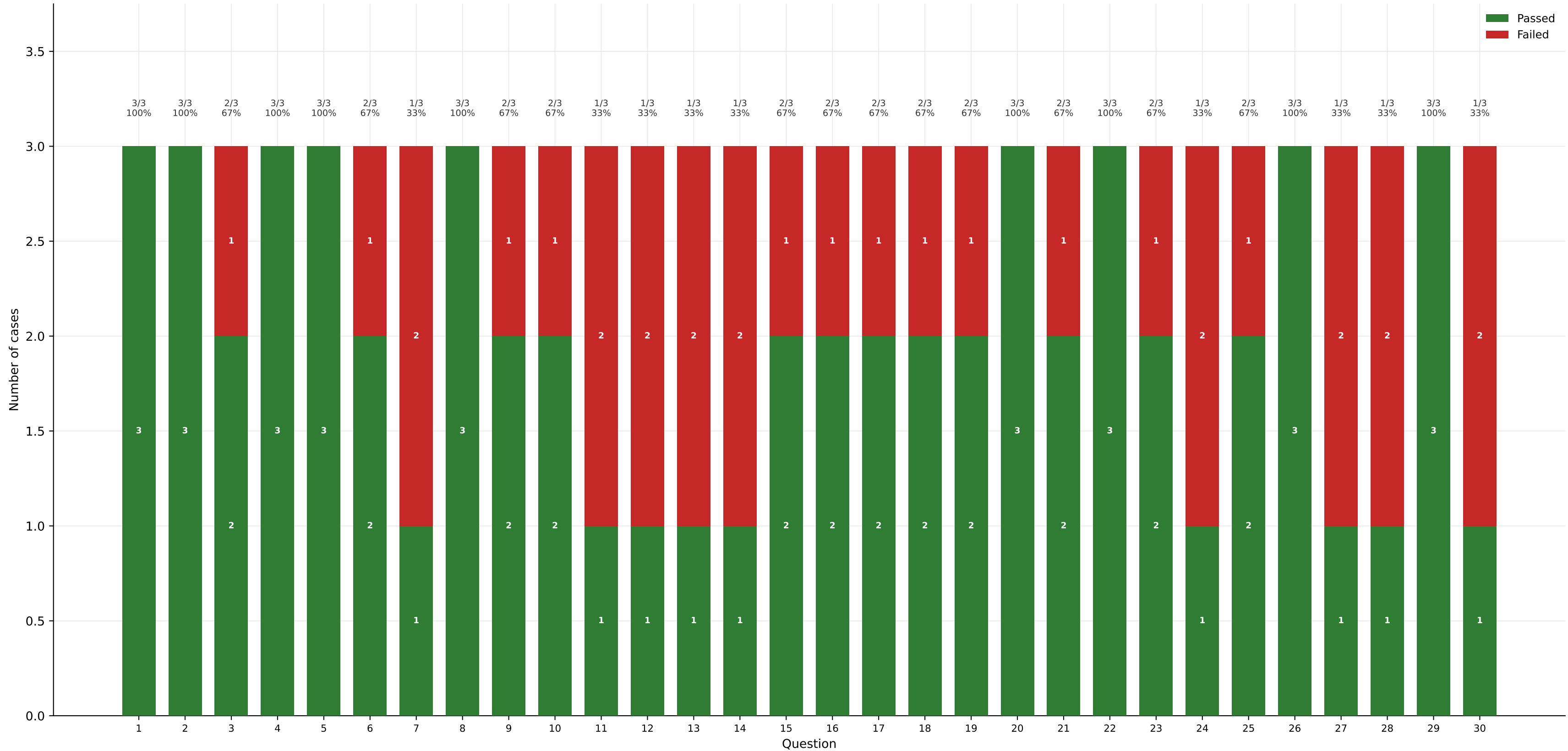
Passed vs failed by question - Claude-Haiku-4.5
