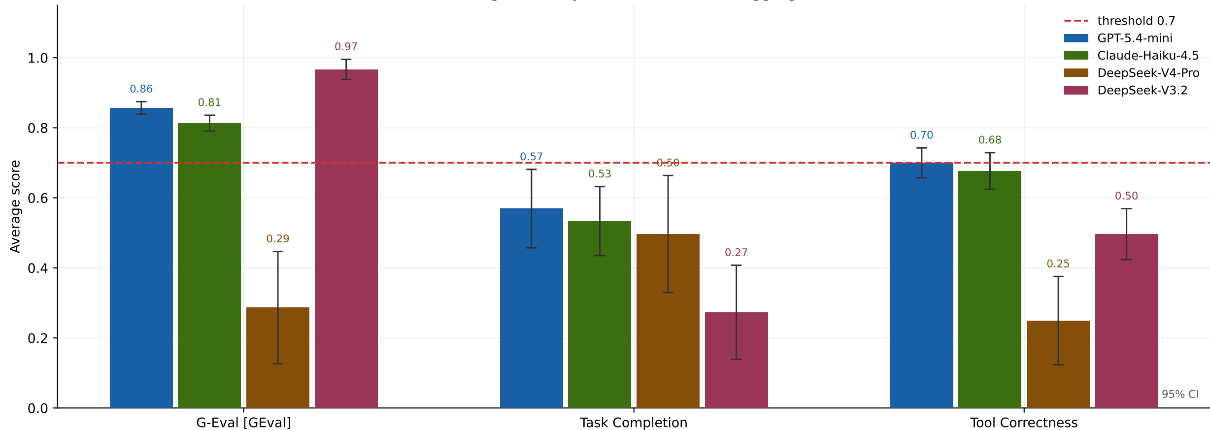
Average score by metric and model - aggregate
