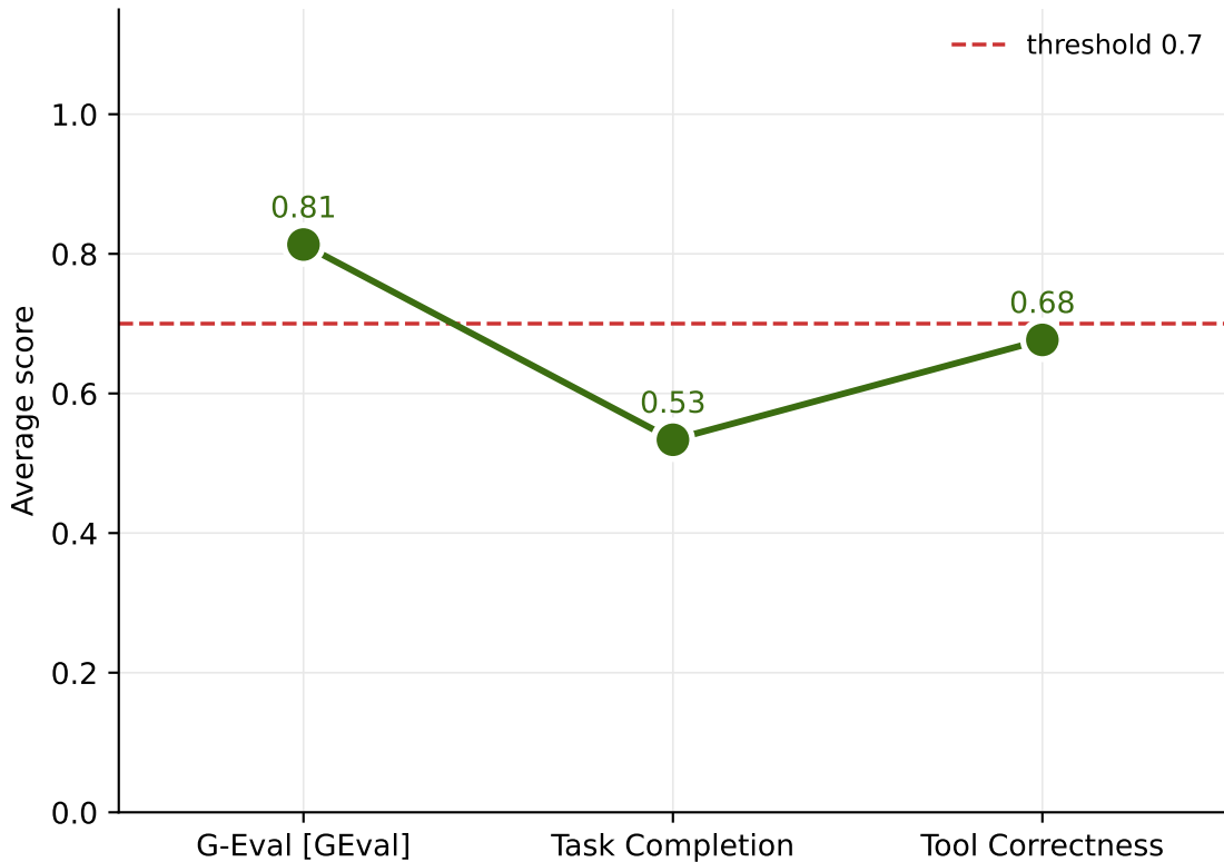
Score by metric - Claude-Haiku-4.5
