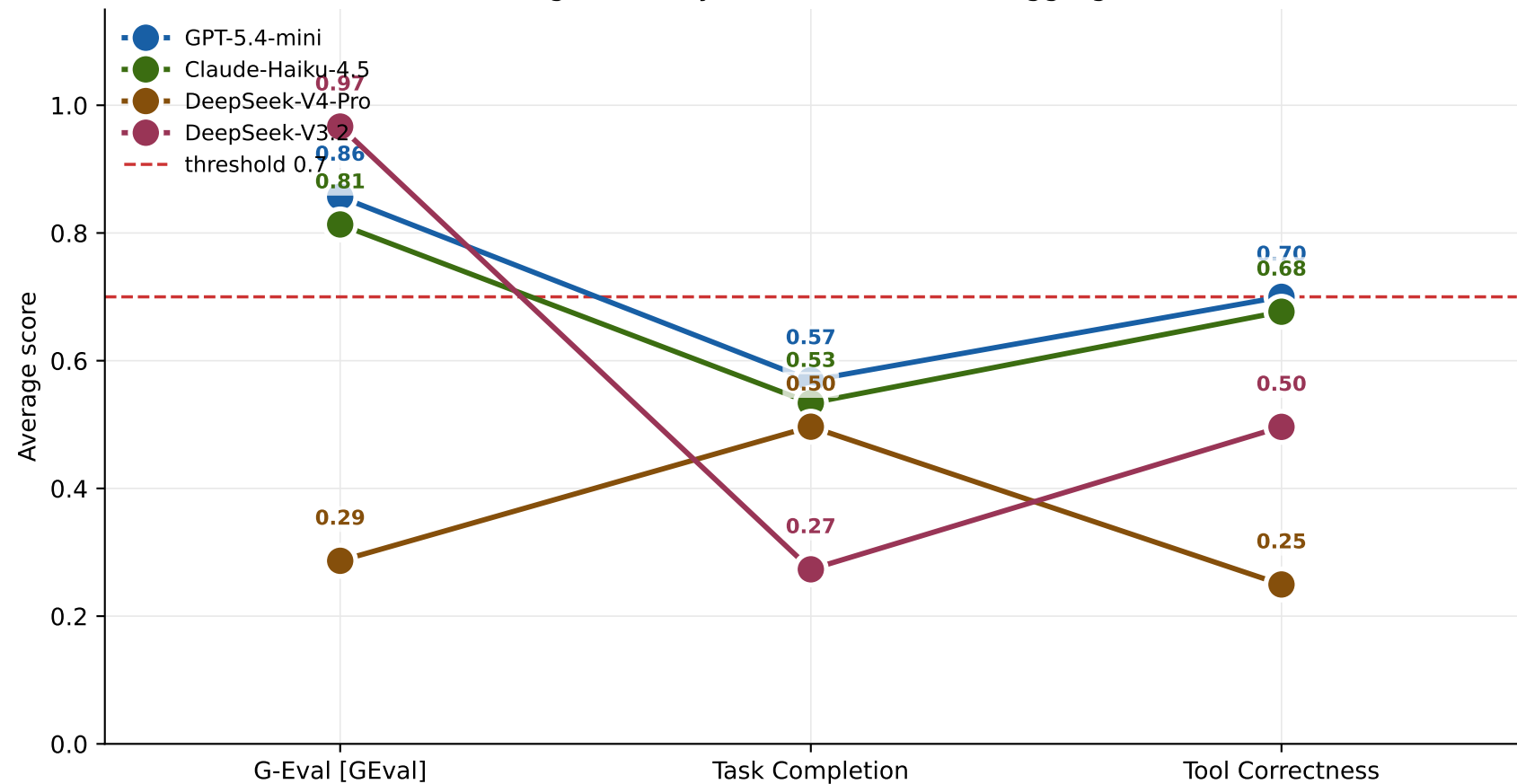
Average score by metric and model - aggregate
