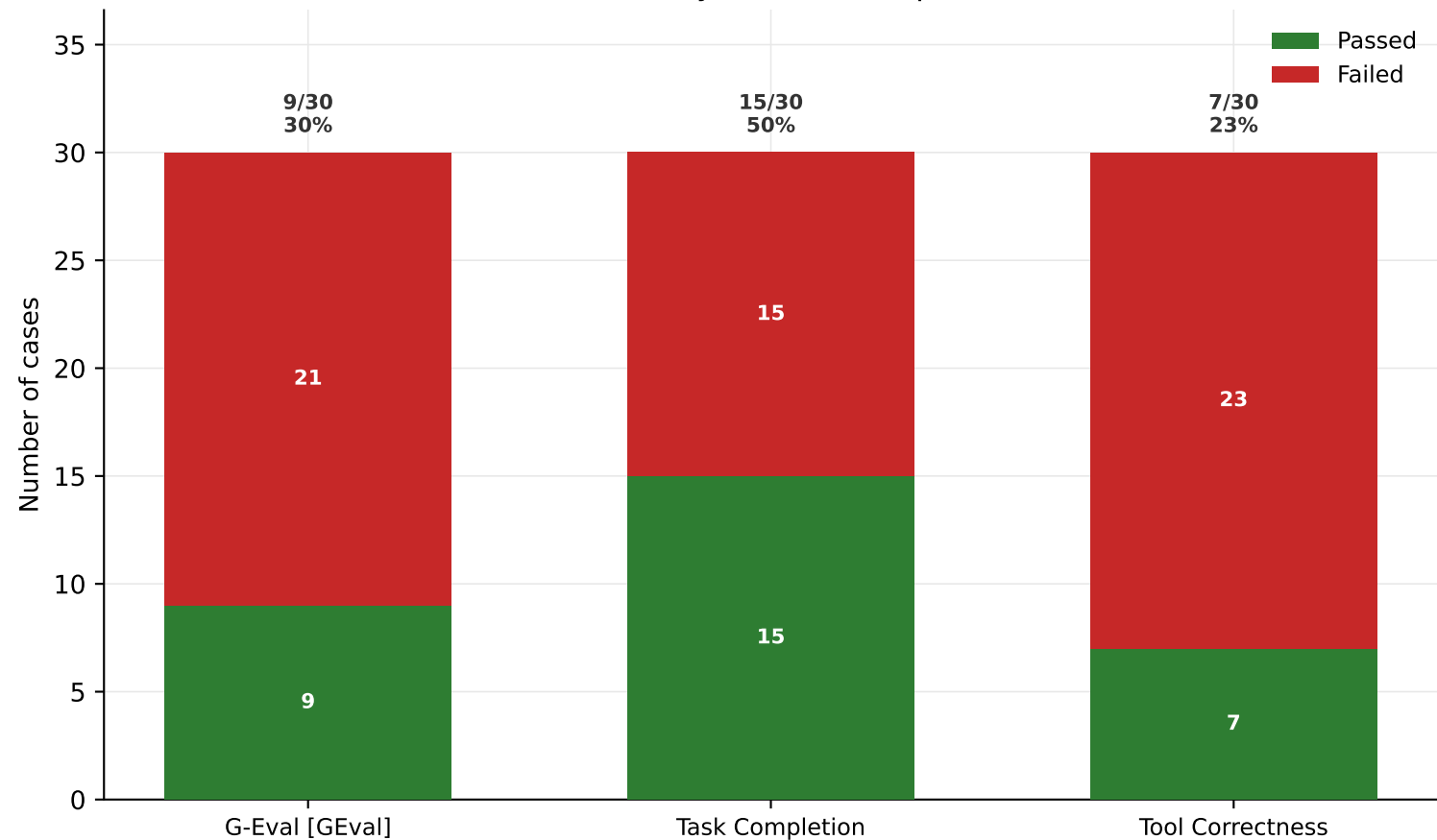
Passed vs failed by metric - DeepSeek-V4-Pro
