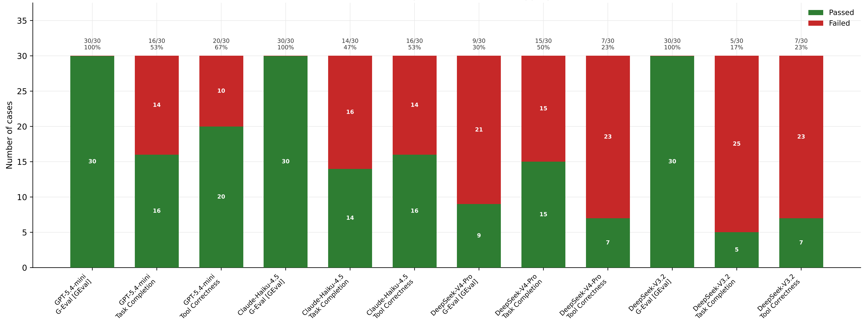
Passed vs failed by metric and model - aggregate
