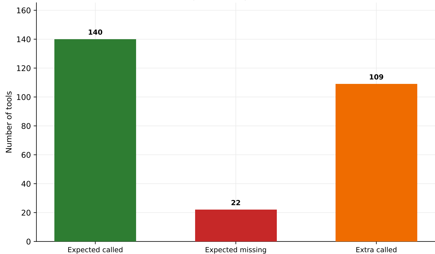
Tool usage summary - GPT-5.4-mini
