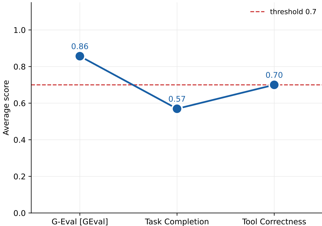
Score by metric - GPT-5.4-mini
