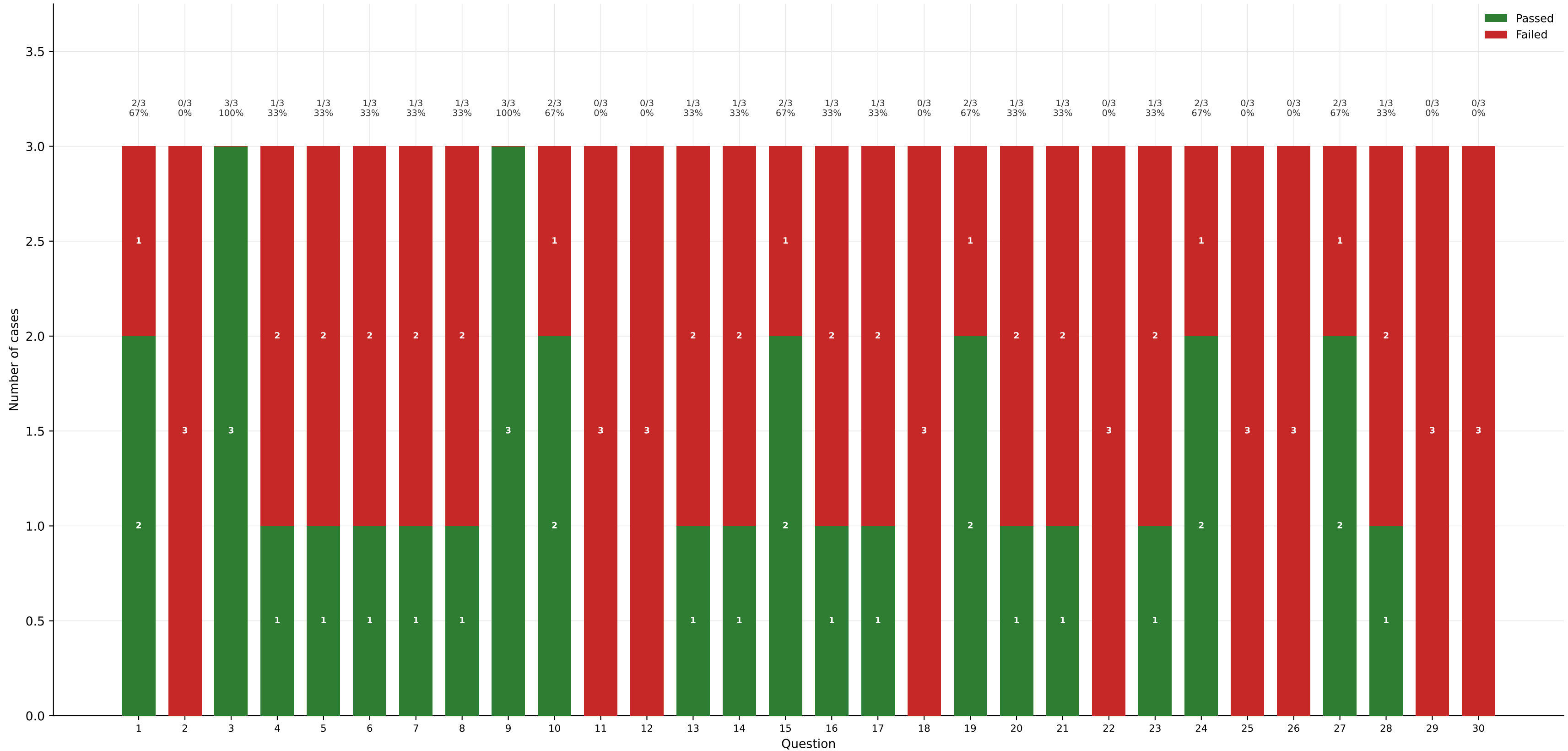
Passed vs failed by question - DeepSeek-V4-Pro
