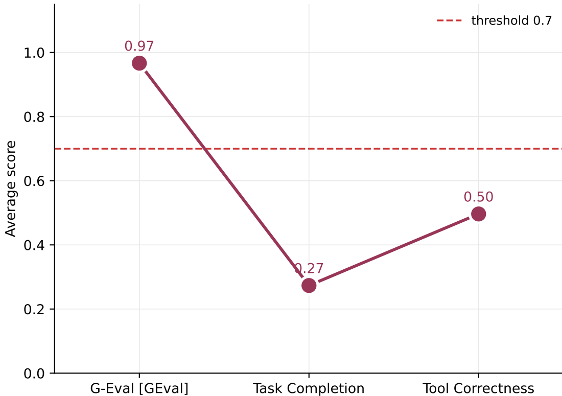
Score by metric - DeepSeek-V3.2
