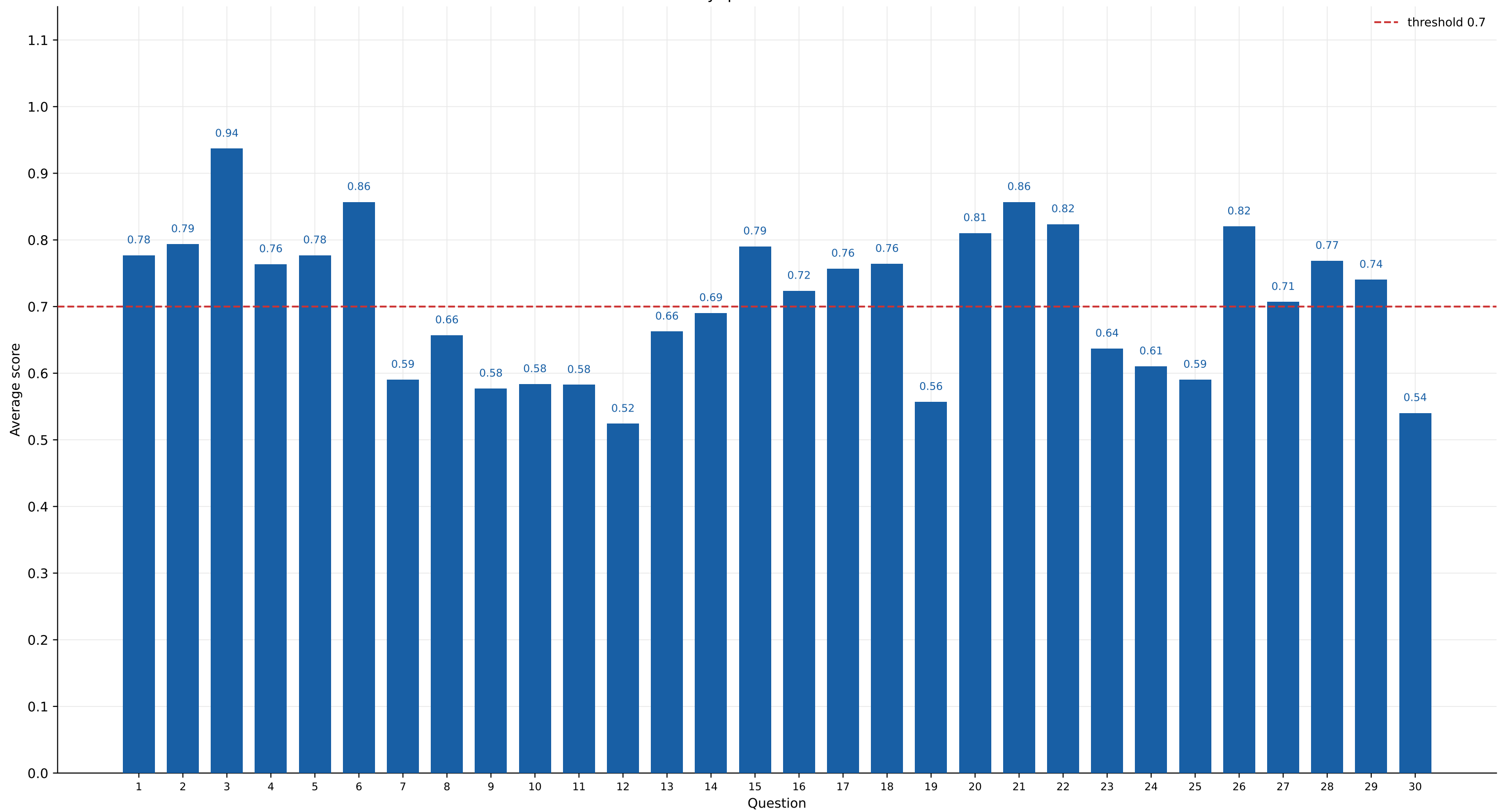
Score by question - GPT-5.4-mini
