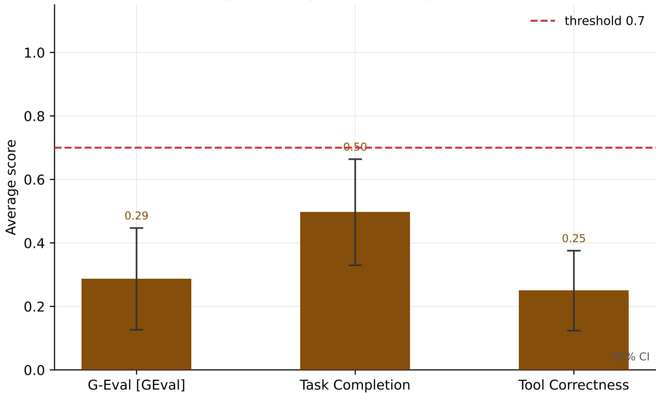
Average score by metric - DeepSeek-V4-Pro
