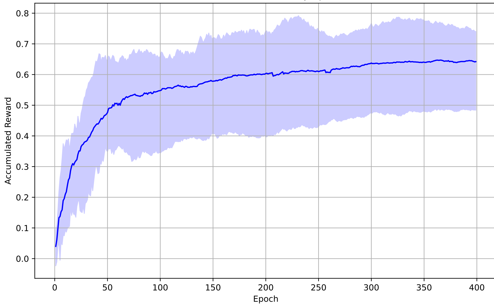
Accumulated Reward by Epoch
