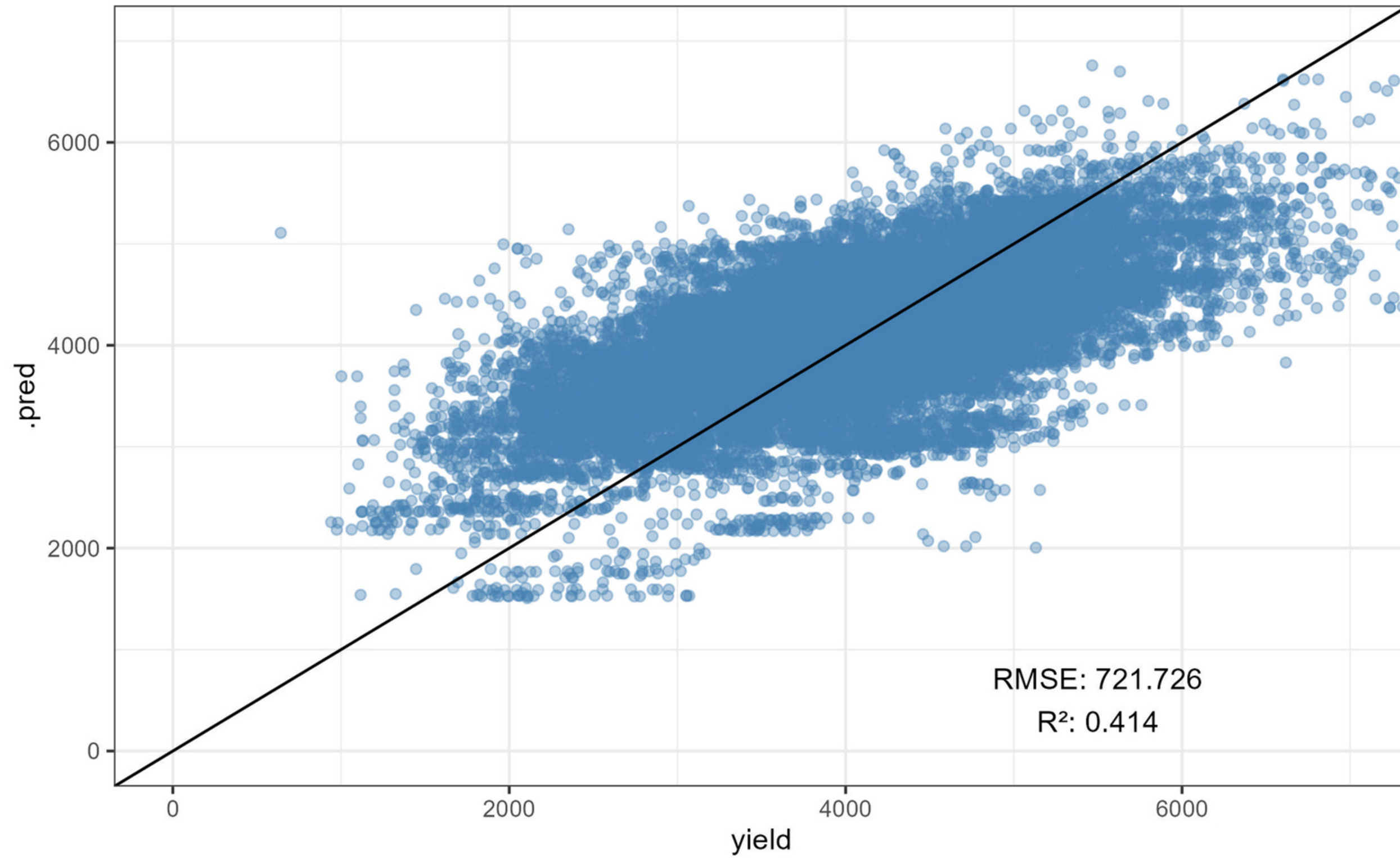
Varieties Test Performance
