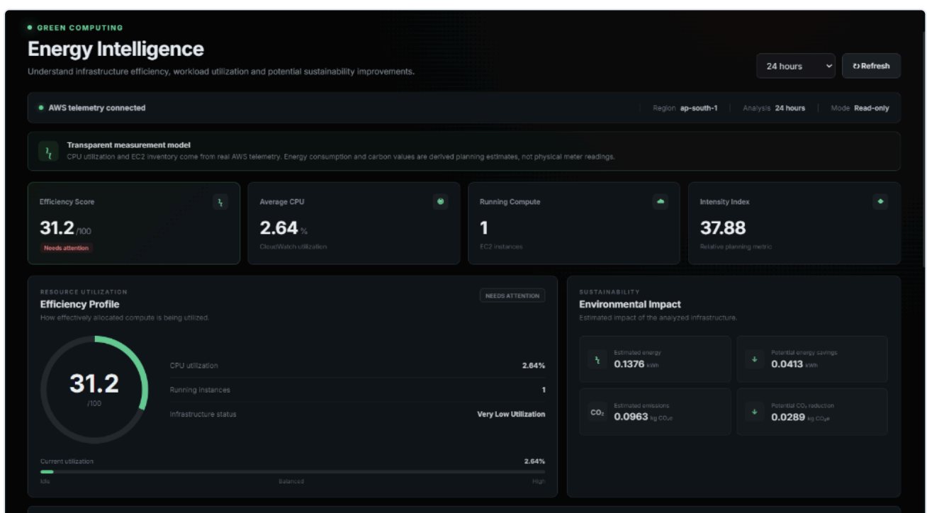
Figure 7.4: Energy Intelligence - Workload Utilization & Environmental Impact
