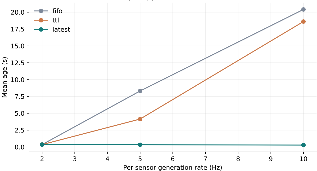
Load sensitivity • application simulation, 16 sensors
