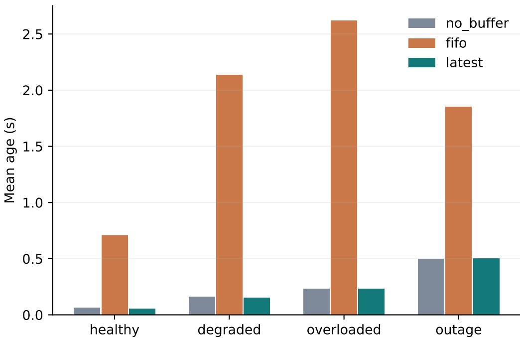
Live-state freshness
