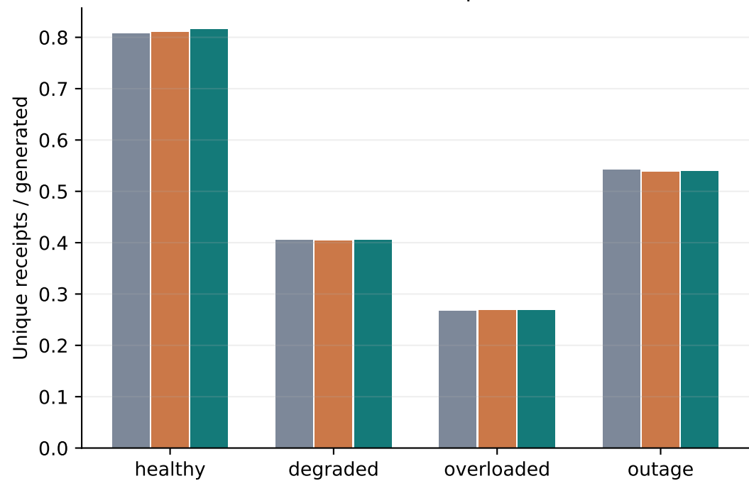
Finite-horizon completeness
