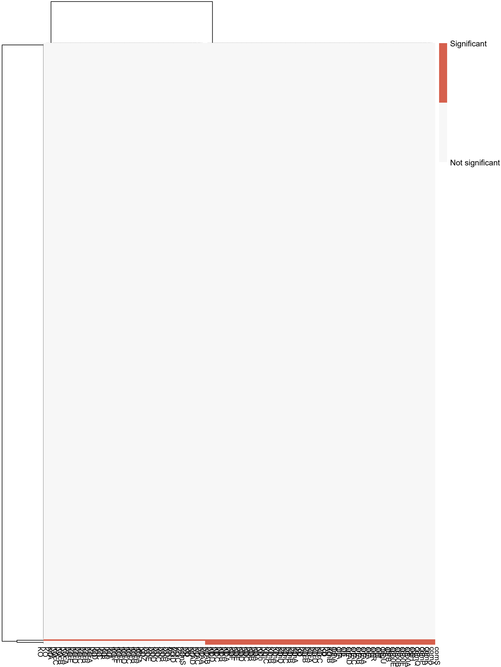
Significance Matrix (1 = significant, p < 0.05 )
