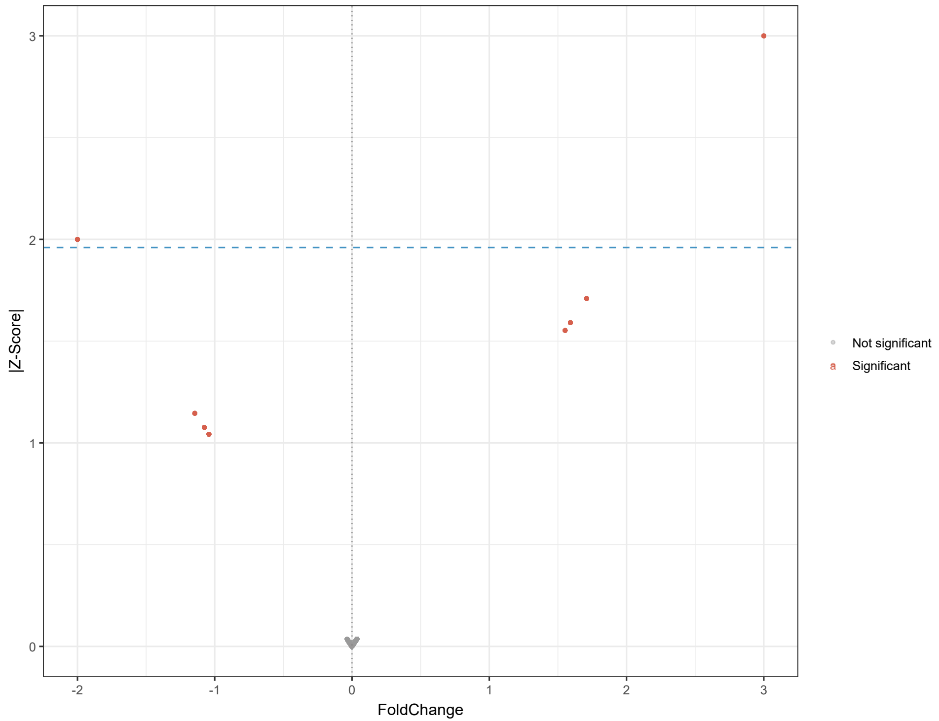
Volcano Plot: FoldChange vs |Z-Score|
