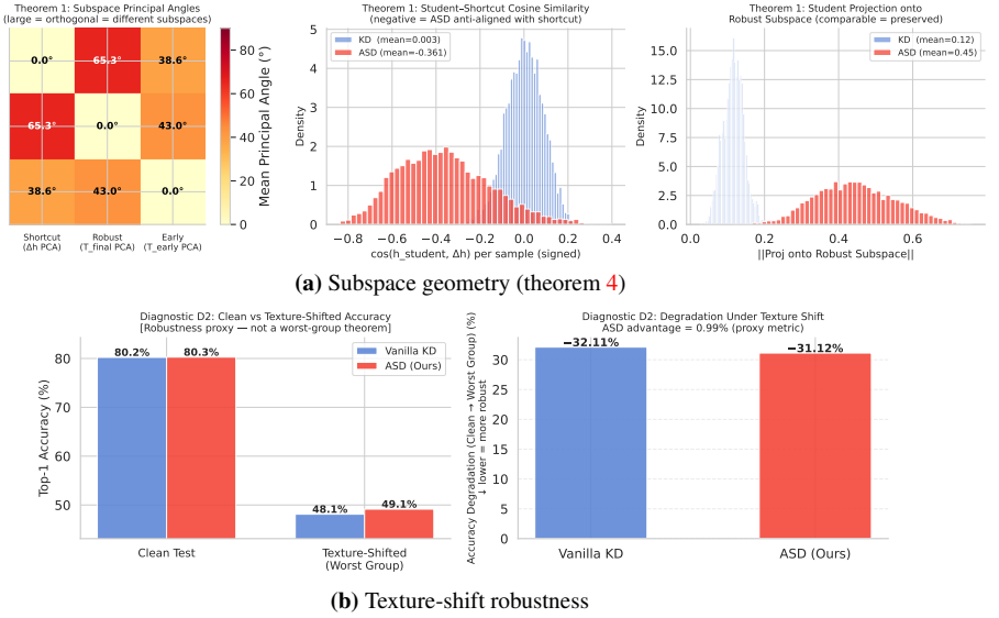
Figure 3: Subspace and robustness diagnostics on P1. ASD separates shortcut directions, improves robust-subspace projection over KD (0.45 vs. 0.12), and slightly reduces texture-shift degradation (−31.12% vs. −32.11%).
