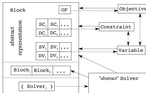
Figure 3: The two faces of a Block : the physical (semantic) data and the abstract Variable / Constraint / Objective representation.
