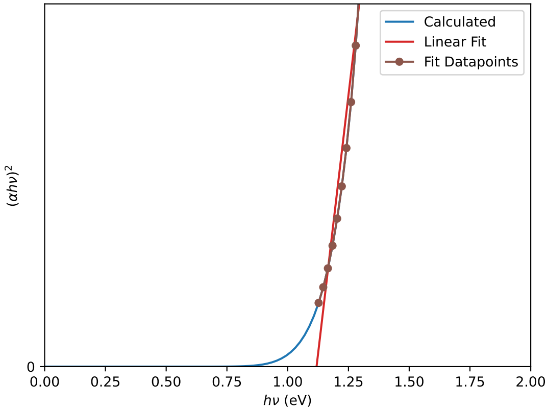
Tauc Plot
