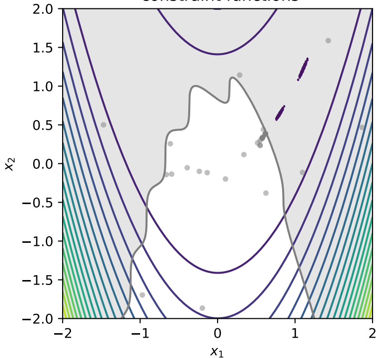
Low-fidelity objective & constraint functions
