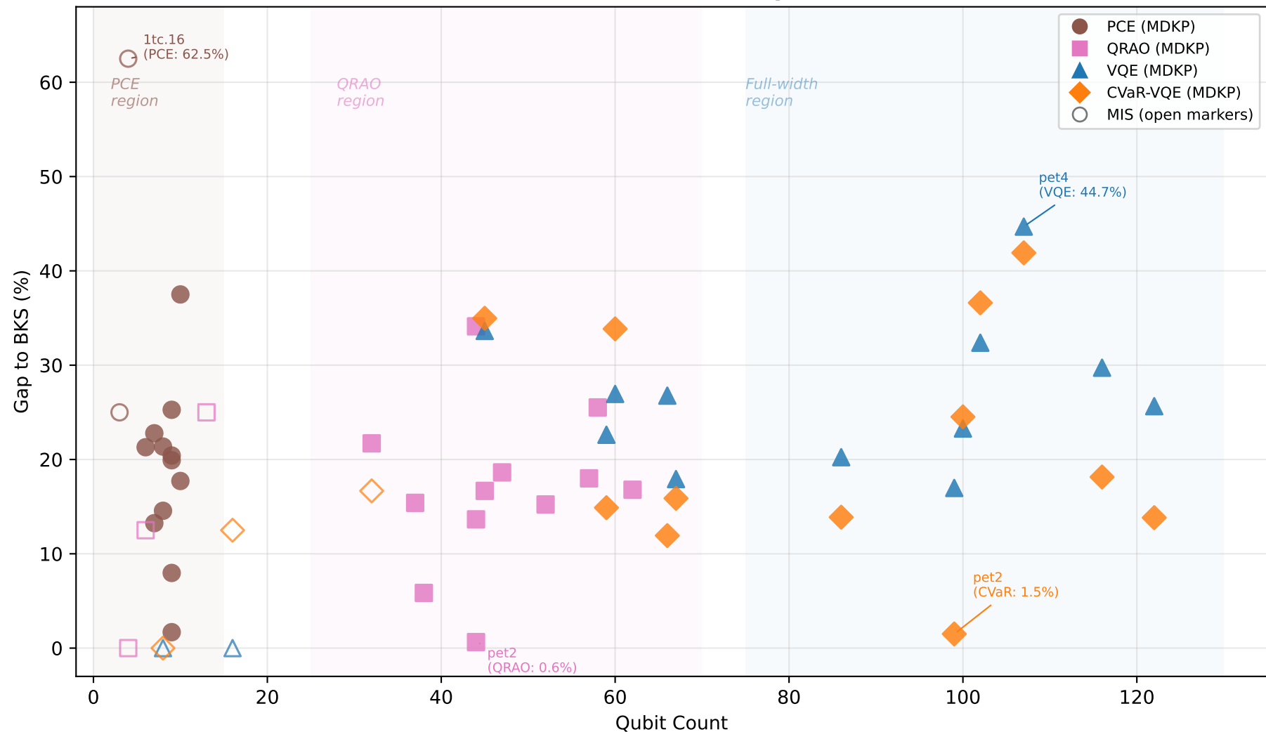
Qubit Count vs. Recovered Solution Quality on Hardware (MDKP: filled markers, MIS: open markers)
