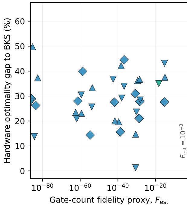
(a) Strongly noise-dominated
