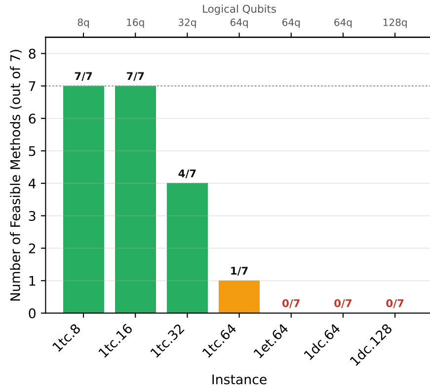
(b) MIS: Feasibility Cliff
