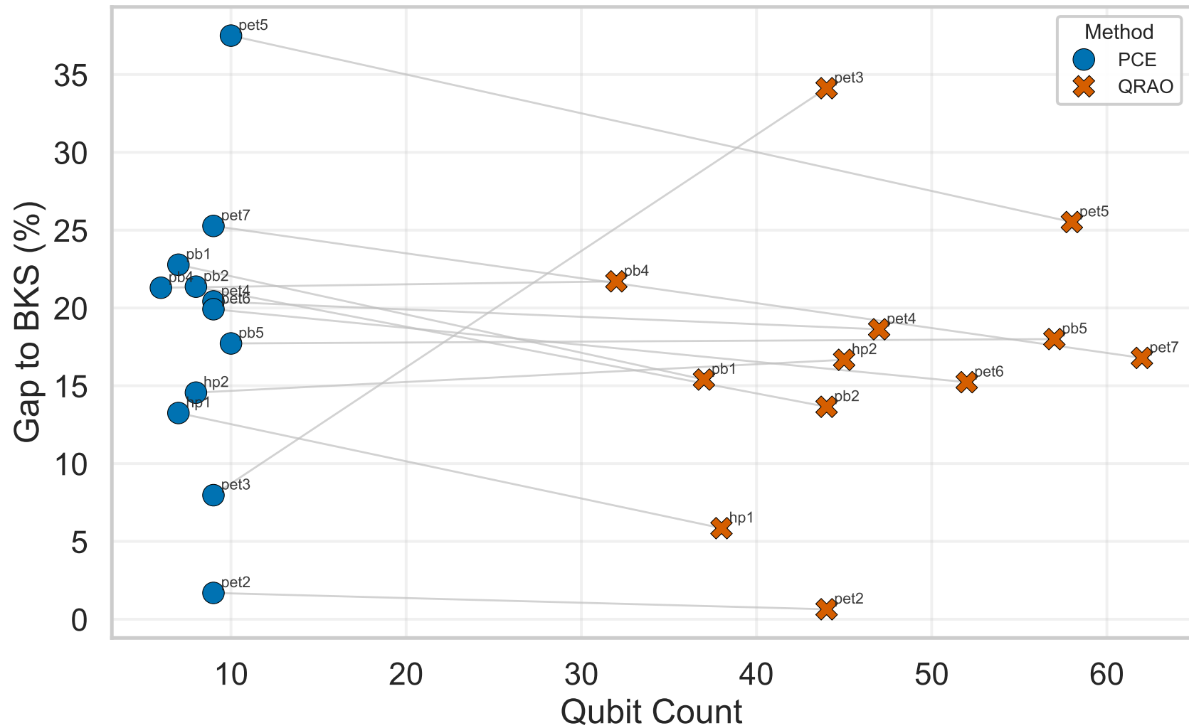
Encoding Tradeoff: Qubits vs Gap (PCE vs QRAO)
