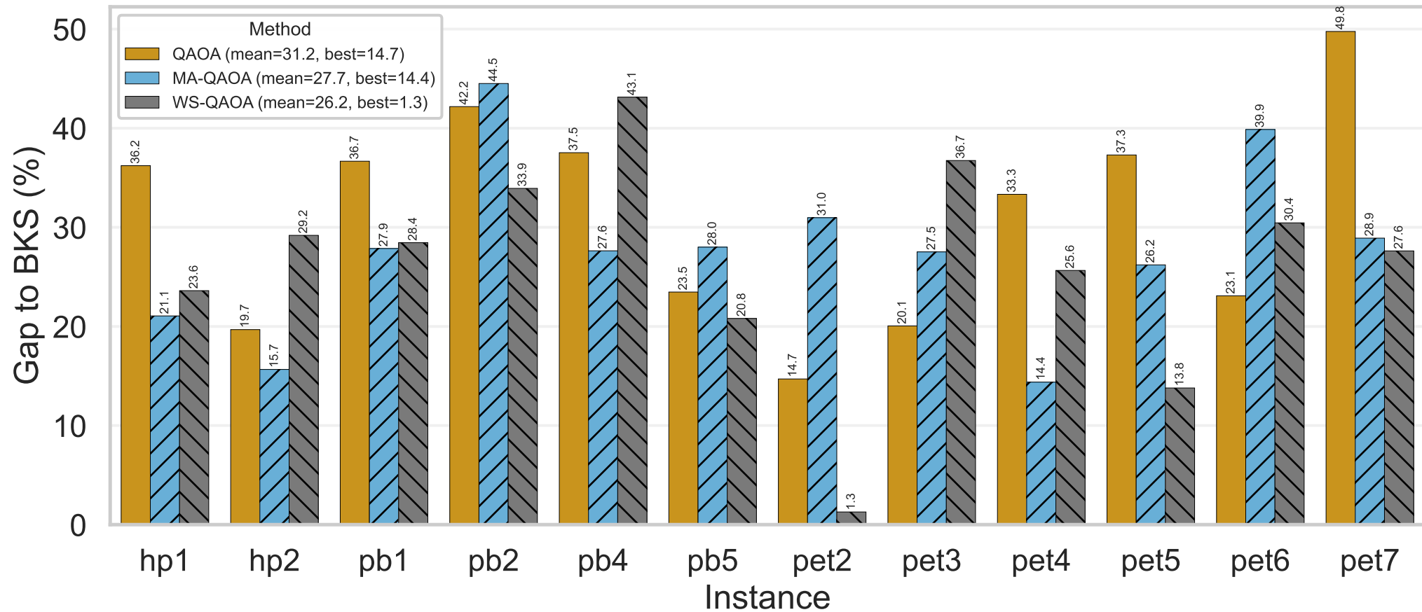
Gap to BKS Across Instances (QAOA Variants)
