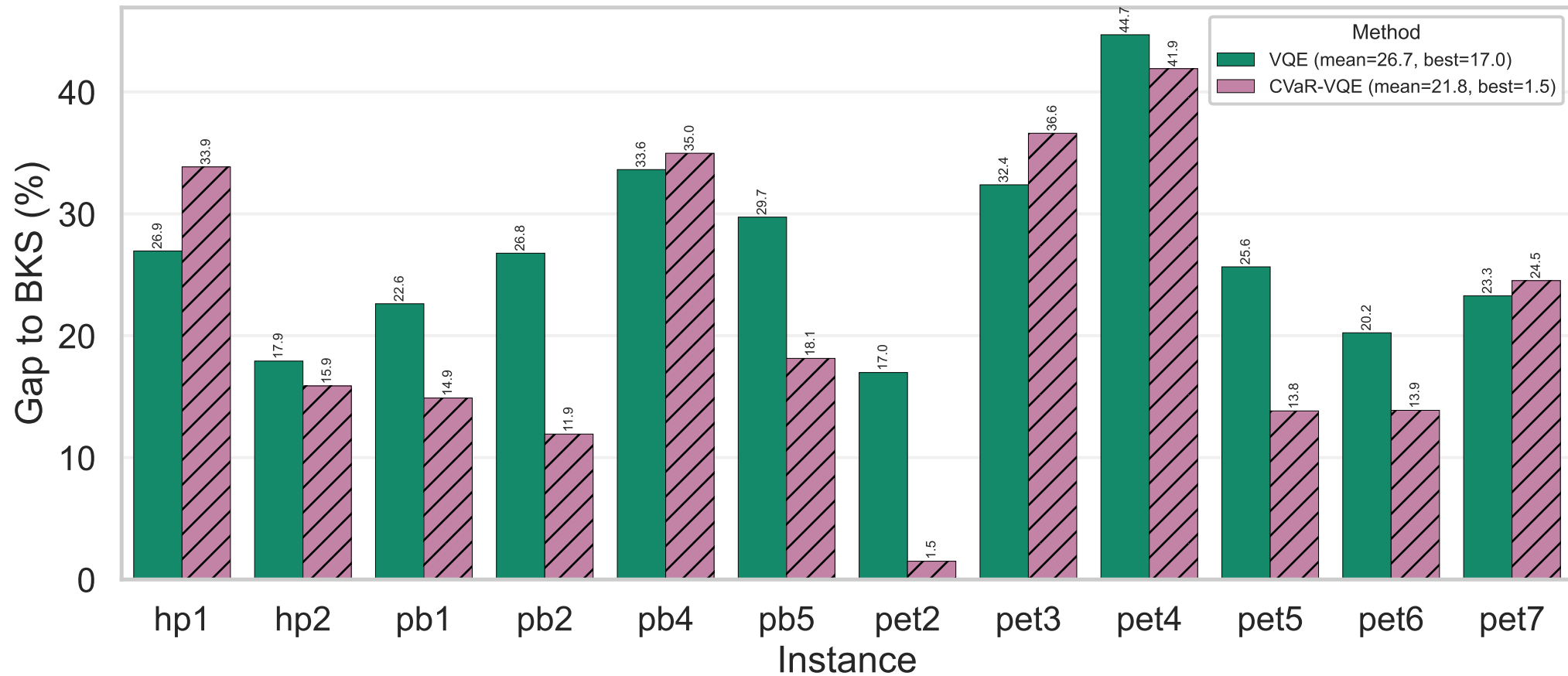
Gap to BKS Across Instances (VQE Variants)
