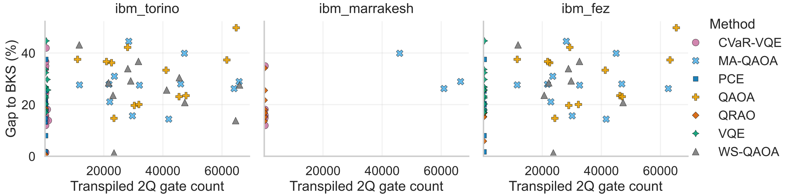
Quality-Cost Scatter: Transpiled 2Q gate count vs Gap
