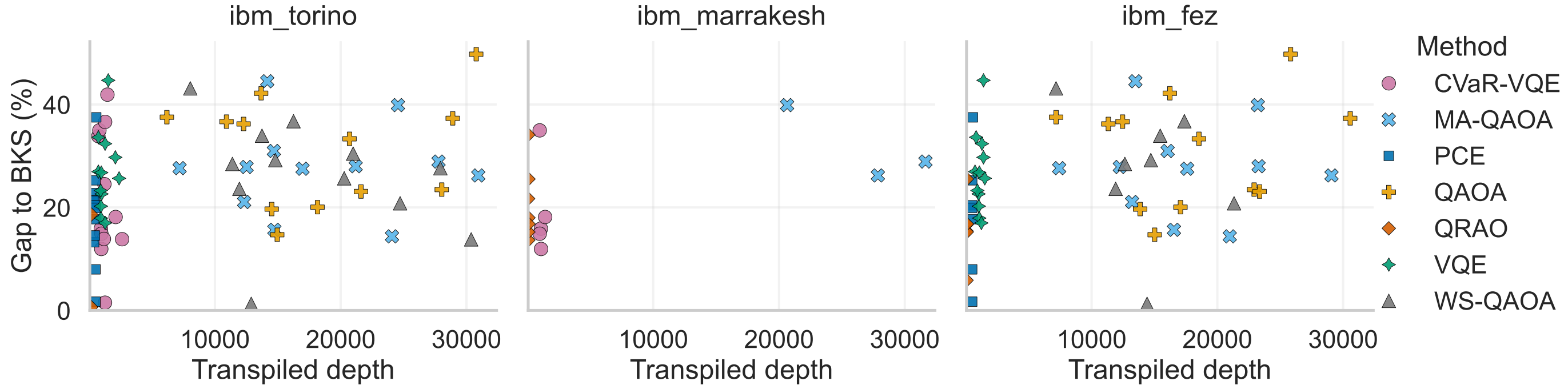
Quality-Cost Scatter: Transpiled depth vs Gap
