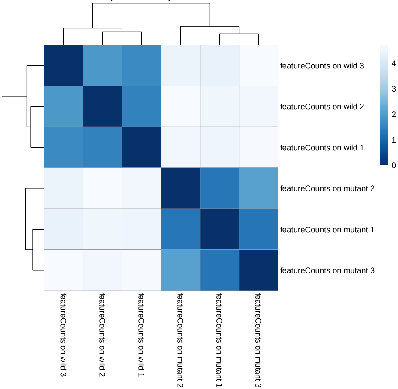
Sample-to-sample distances
