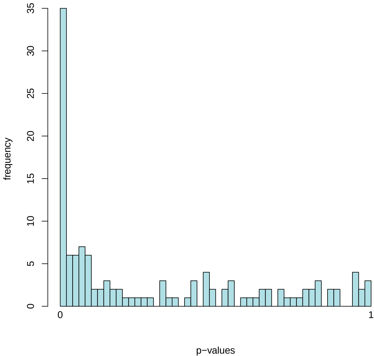
Histogram of p-values for Condition: Wild vs Mutant
