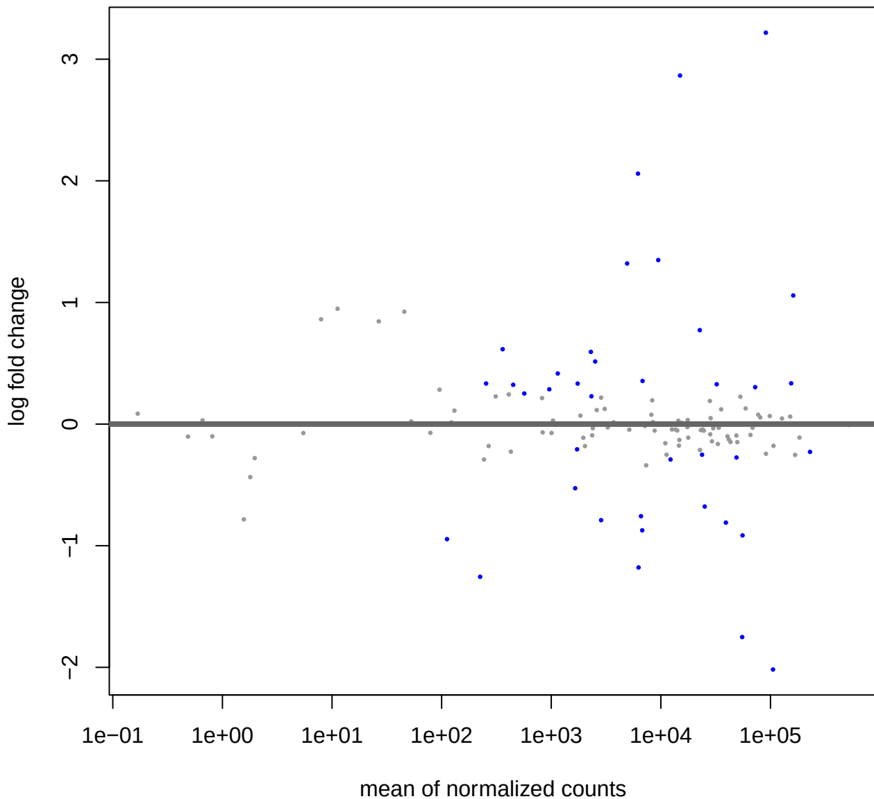
MA-plot for Condition: Wild vs Mutant
