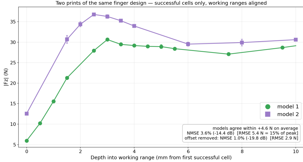
Figure 5.3: Contact force versus calibrated depth for two independently printed copies of finray_18 , zero tilt, successful cells only. Error bars: one standard deviation across repeats.
