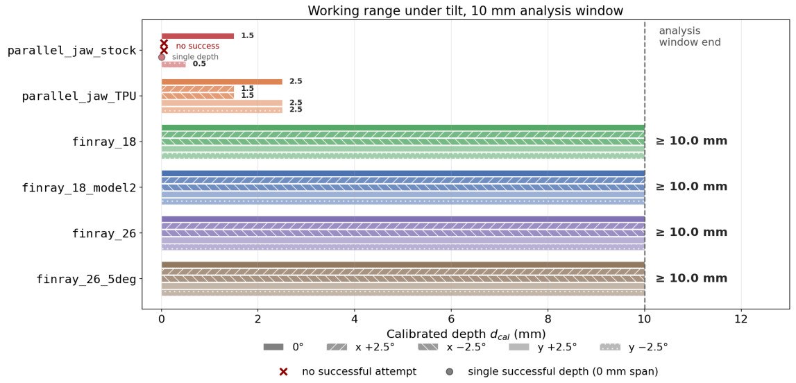
Figure 5.6: Successful-grasp working range on the calibrated depth axis, all five tested orientations per variant. \times : no successful attempt at any depth. Hatched bars are right-censored at the analysis-window end.
