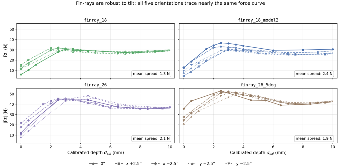
Figure 5.2: Contact force versus calibrated depth for each finray variant, all five tested orientations overlaid ( 0^\circ , x \pm 2.5^\circ , y \pm 2.5^\circ ). Within each panel the five curves nearly coincide.
