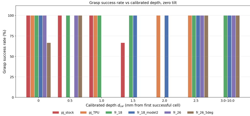
Figure 5.4: Grasp success rate versus calibrated depth, zero tilt, binned in 0.5 mm increments below 3 mm and pooled above. \times : 0% success.
