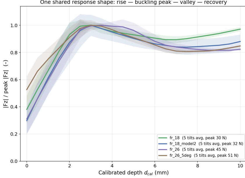
Figure 5.1: Peak-normalised |F_z| versus calibrated depth d_{\text{cal}} , averaged over all five tested orientations per variant (shaded band: across-orientation spread). All four finray variants collapse onto one shared response shape.
