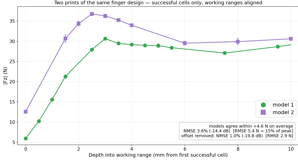
Figure 5.2: Contact force versus calibrated depth for two independently printed copies of finray_18 , zero tilt, successful cells only. Error bars: one standard deviation across repeats.
