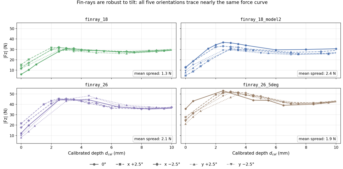
Figure 5.5: Contact force versus calibrated depth for each finray variant, all five tested orientations overlaid ( 0^\circ , x \pm 2.5^\circ , y \pm 2.5^\circ ). Within each panel the five curves nearly coincide.
