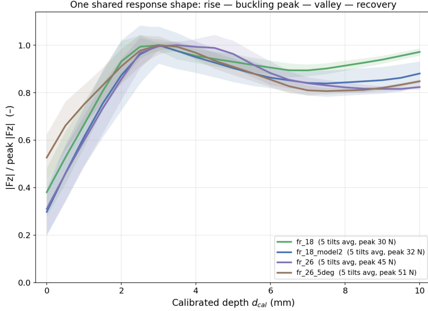
Figure 5.6: Peak-normalised |F_z| versus calibrated depth d_{\text{cal}} , averaged over all five tested orientations per variant (shaded band: across-orientation spread). All four finray variants collapse onto one shared response shape.
