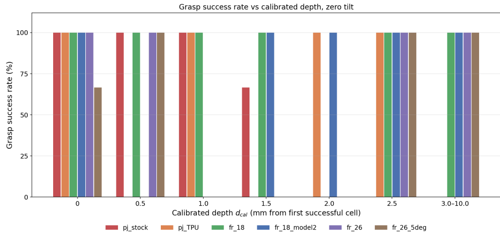
Figure 5.7: Grasp success rate versus calibrated depth, zero tilt, binned in 0.5 mm increments below 3 mm and pooled above. \times : 0% success.
