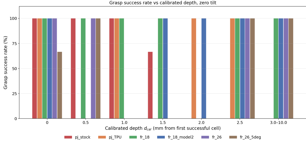
Figure 5.6: Grasp success rate versus calibrated depth, zero tilt, binned in 0.5 mm increments below 3 mm and pooled above. \times : 0% success.
