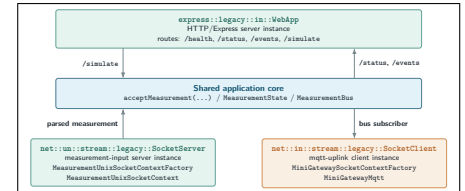
fig-12-minigateway-extended-instance-architecture.pdf
