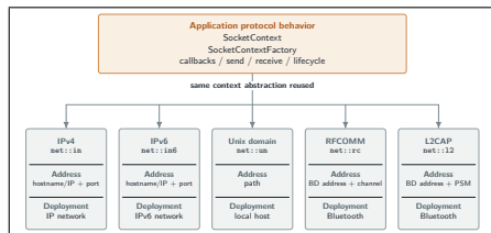
fig-04-lower-family-transfer-model.pdf
