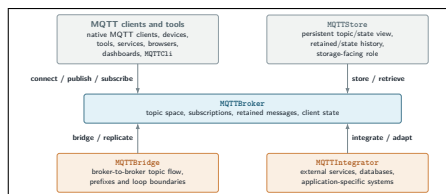
fig-10-mqttsuite-ecosystem-map.pdf
