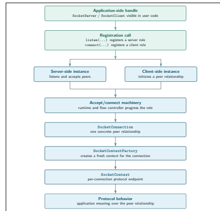
fig-05-server-client-connection-context-path.pdf
