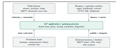
fig-08-iot-boundary-constellation.pdf
