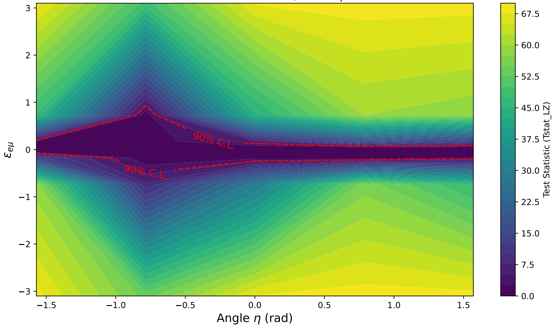
LZ (2025) Sensitivity for \varepsilon_{e\mu}
