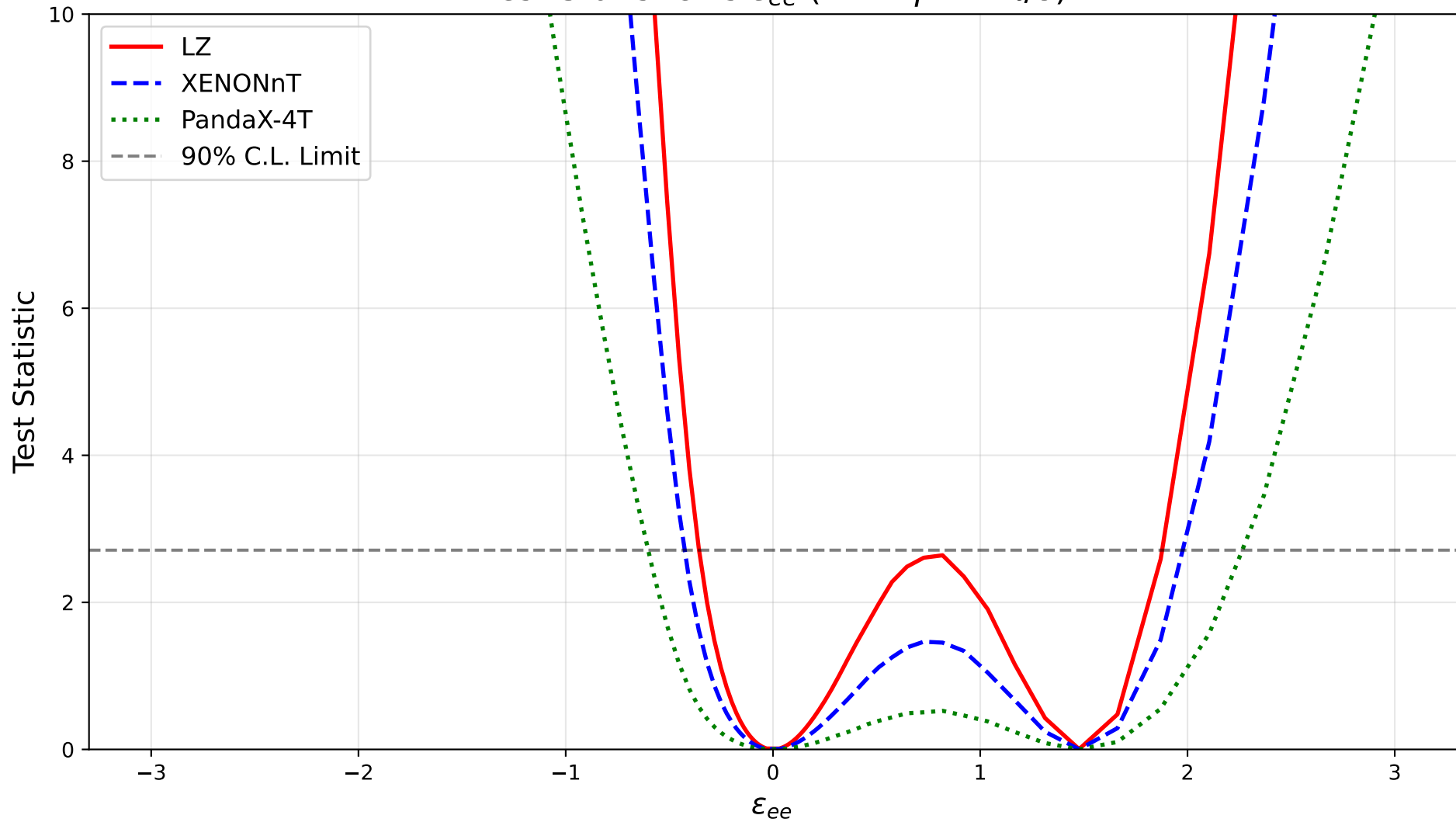
Test Statistic vs \varepsilon_{ee} (with \eta = -\pi/8 )
