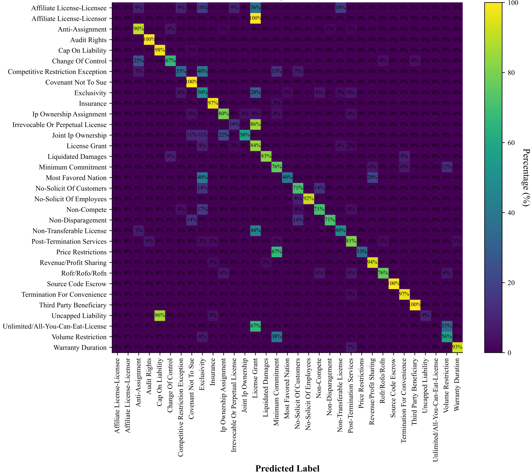
Confusion Matrix – Proposed Hybrid SVM+DBRT
