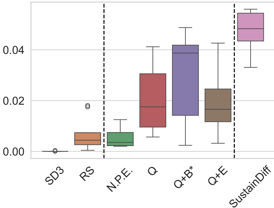
Hypervolume Score
