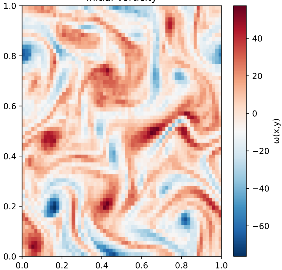
Initial Vorticity
