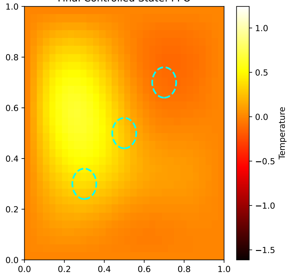
Final Controlled State: PPO
