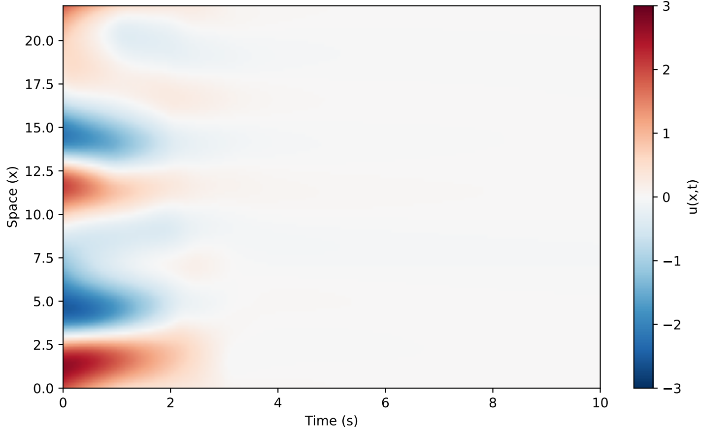
Controlled State: PPO
