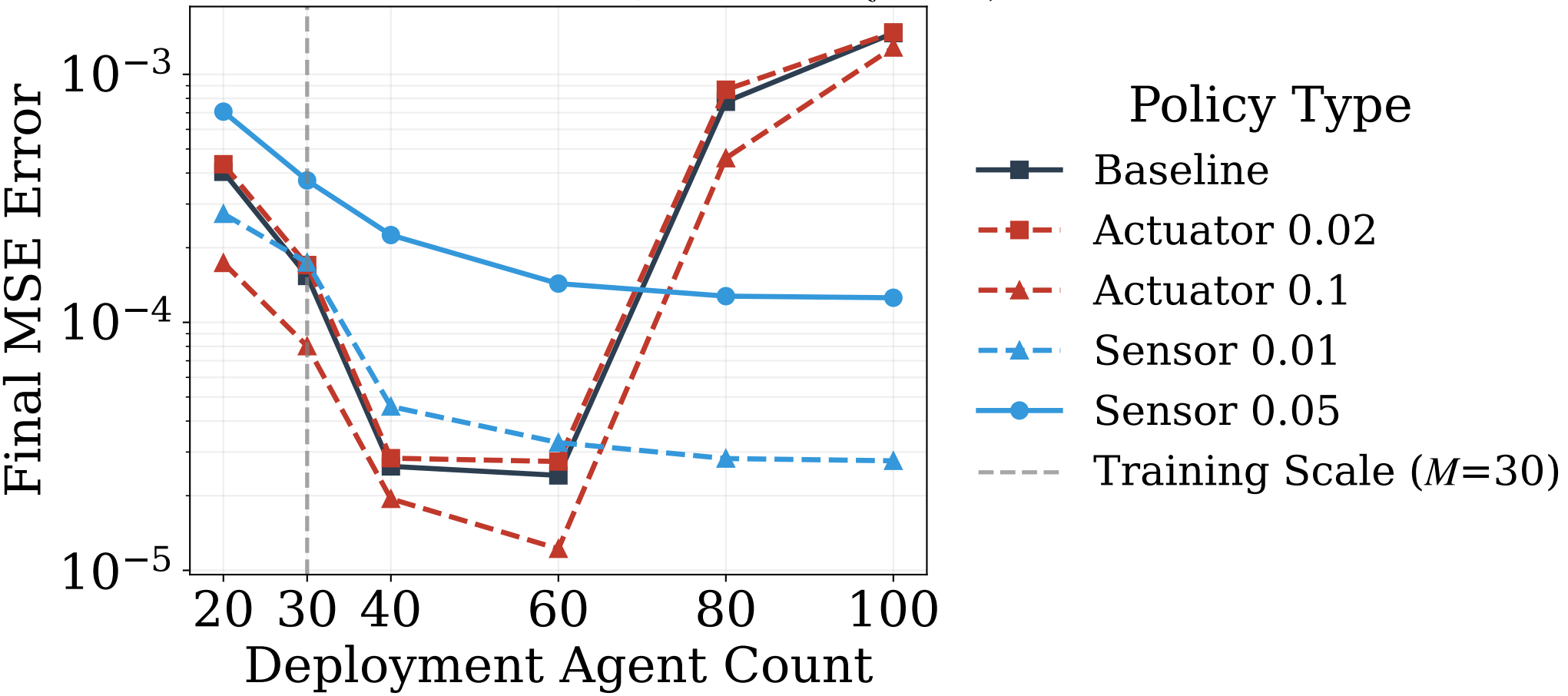
Low Actuator Noise ( \sigma_u = 0.02, \sigma_z = 0.0 )
