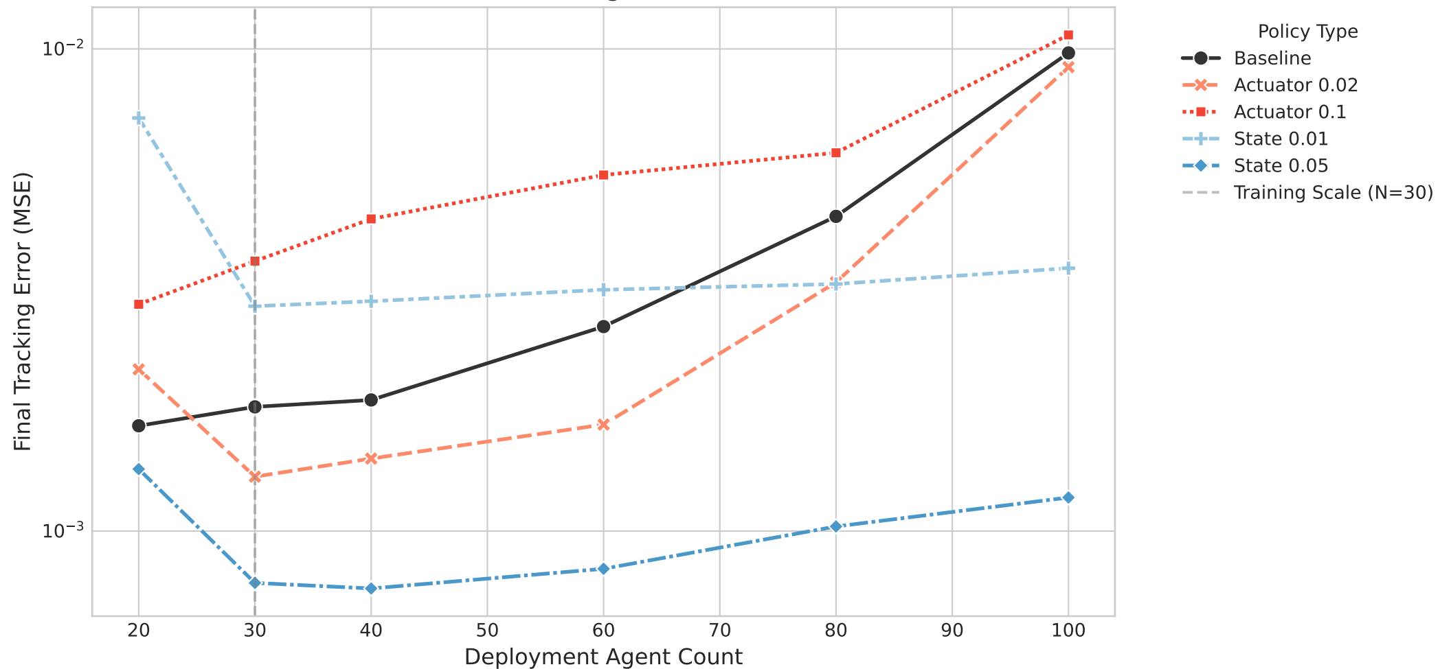
Robustness in Actuator High Env ( \sigma_u = 0.5, \sigma_z = 0.0 )
