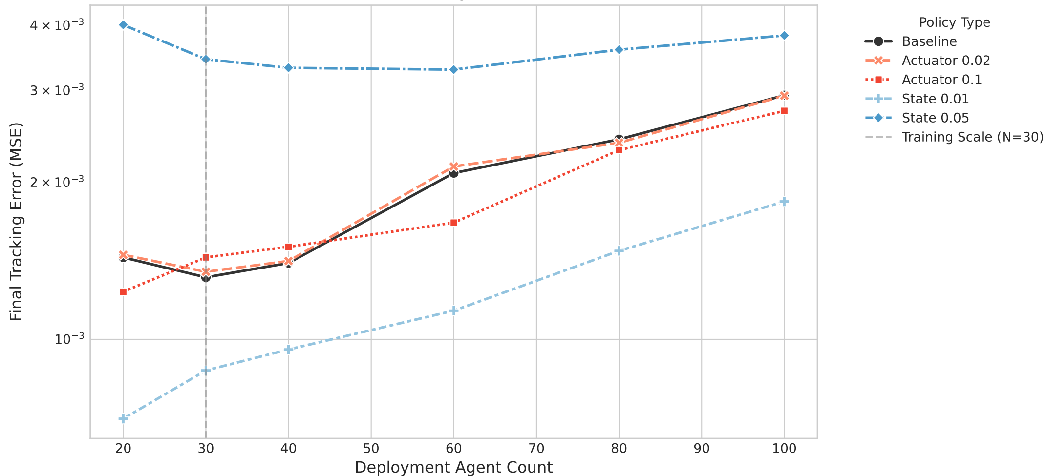
Robustness in Combined High Env ( \sigma_u = 0.5, \sigma_z = 0.25 )
