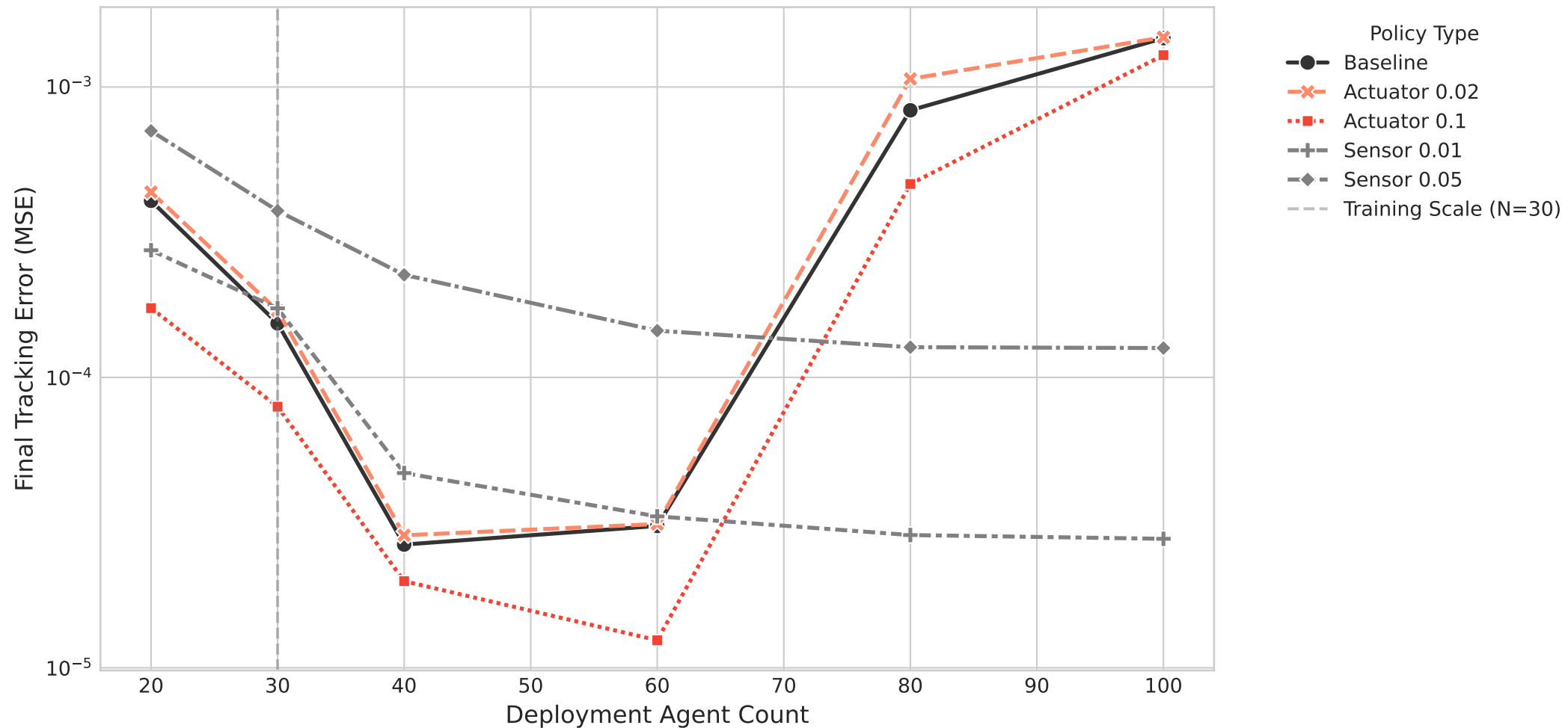
Robustness in Actuator Mid Env ( \sigma_u = 0.1, \sigma_z = 0.0 )
