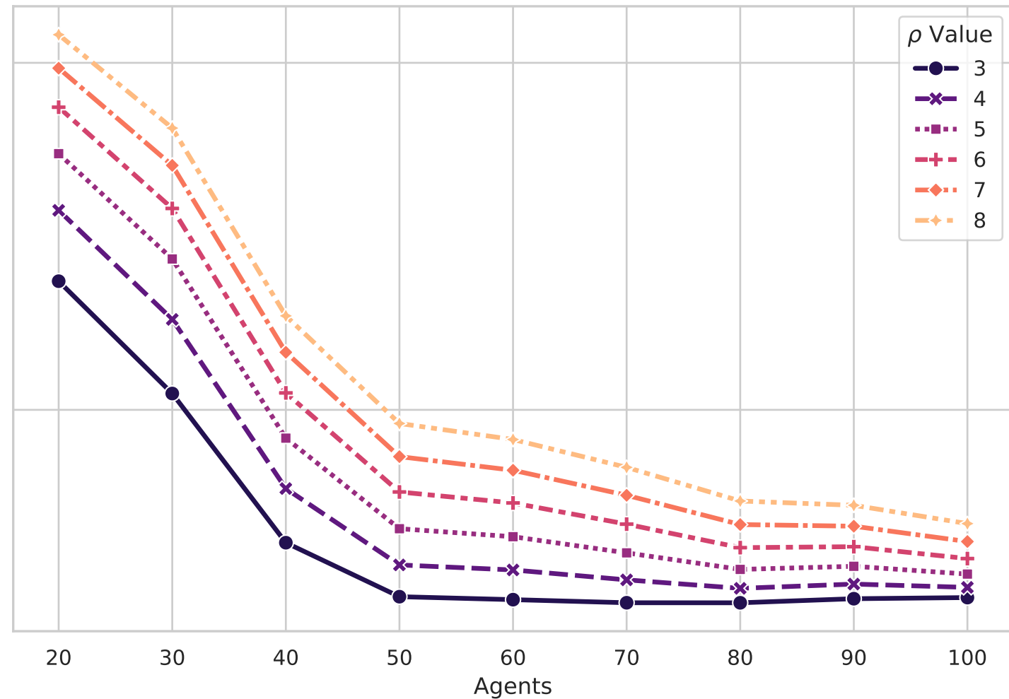
Sensitivity to Growth Rate ( \rho ). \rho_{\text{for training}} \text{ is } 3.0 Fixed \nu = 0.005
