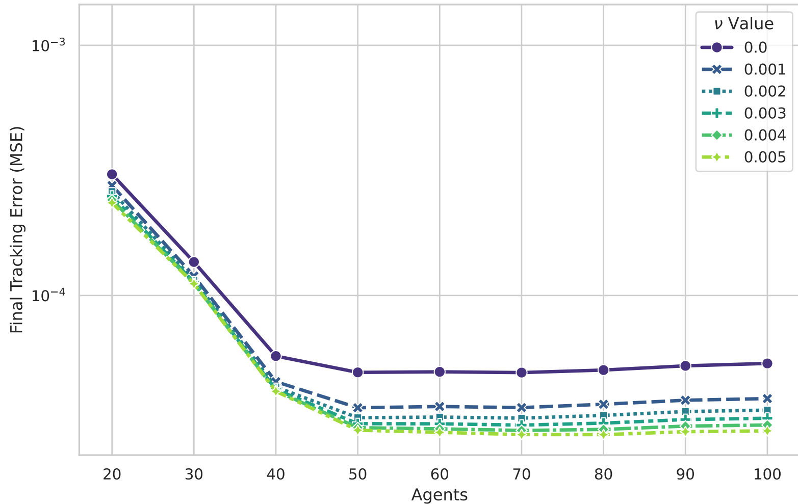
Sensitivity to Diffusion ( \nu ). \nu_{\text{for training}} \text{ is } 0.005 Fixed \rho = 3.0
