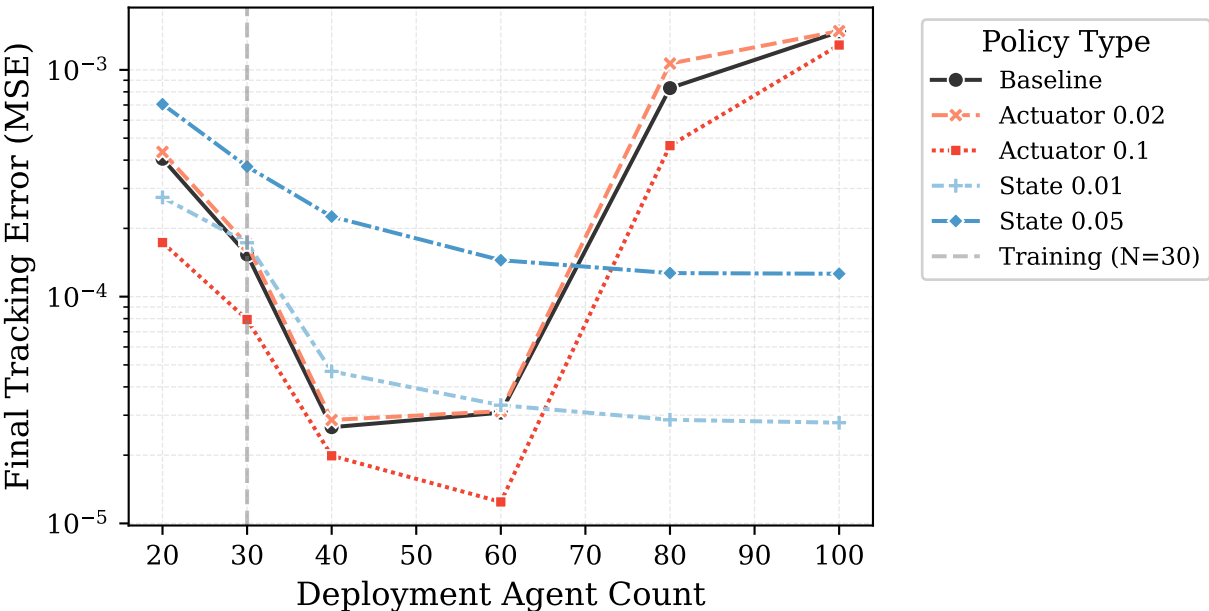
Robustness: Actuator Mid ( \sigma_u=0.1, \sigma_z=0.0 )
